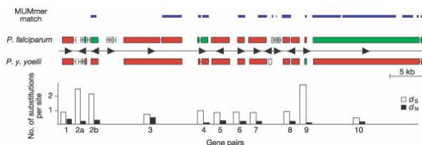
Figure 7. Global alignment scheme of a syntenic region between P. falciparum and P. yoeli encompassing ten orthologous gene pairs and nine intergenic regions
