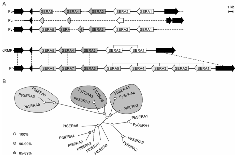
Figure 1. Deduced organization of the cRMP SERA locus
