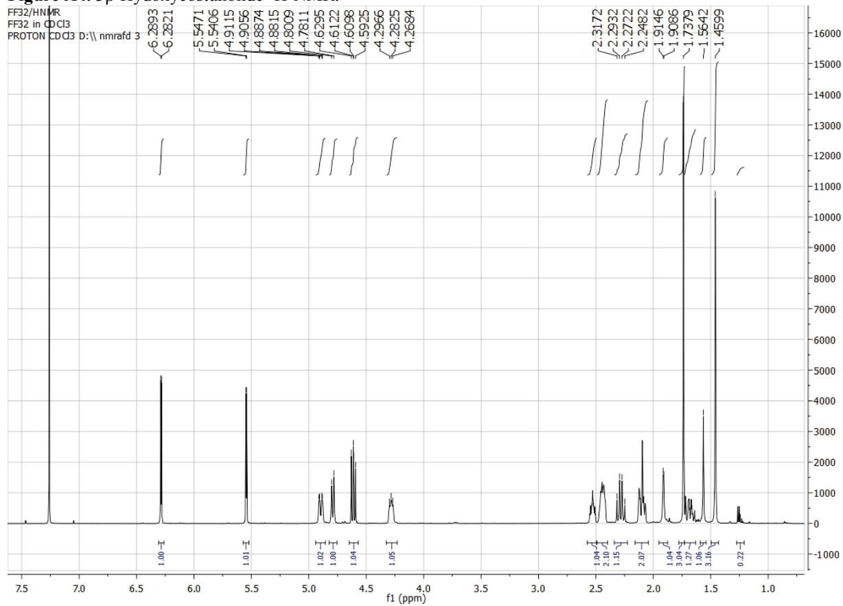
Figure A4. 3 \beta -Hydroxycostunolide 1 H-NMR.
