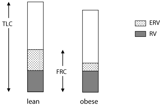
Figure 2 Altered lung function in obesity Obesity leads to alternations of lung volumes. ERV: expiratory reserve volume; FRC: functional residual capacity; RV: residual volume; TLC: total lung capacity
