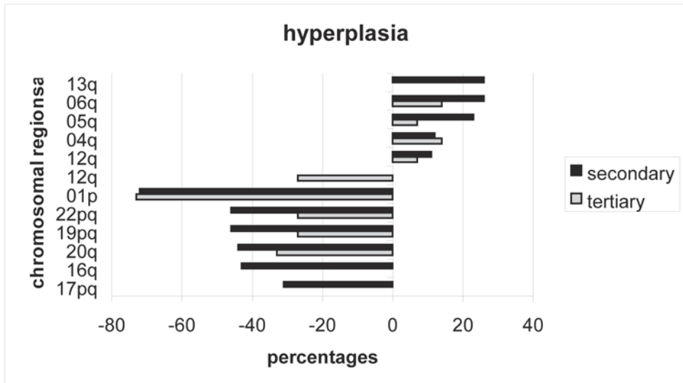
Figure 2 A, B and C depict the regions frequently (in >10% of cases) lost and gained in carcinomas (A) ,adenomas (B) and hyperplasia (C) found by CGH analysis. 3;4;20;32;39 . In C percentages of gains and losses are indicated in a similar way as in A/B.
