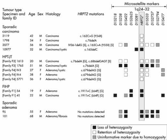
Figure 1 Mutations detected within HRPT2 , and LOH analysis of flanking markers. "Age" is the age in years at the time of parathyroidectomy. HRPT2 mutations detected are listed as nucleotide changes and amino acid changes where relevant. Where two mutations were detected in the same patient, both are listed. Germline mutations are denoted "[G]", and somatic mutations are denoted "[S]". For the microsatellite markers, see key in figure. Blank spaces indicate LOH testing not performed (germline DNA not available). *The approximate location of HRPT2 within the 1q24-32 region. The results in this shaded column represent retention or loss of heterozygosity at the HRPT2 locus by combined microsatellite and intragenic mutation results. †D1S218 and D1S477 have been reported previously. 31 ‡Previously reported as having LOH at 1q and 1p and CGH loss at 1q31-qter. 34
