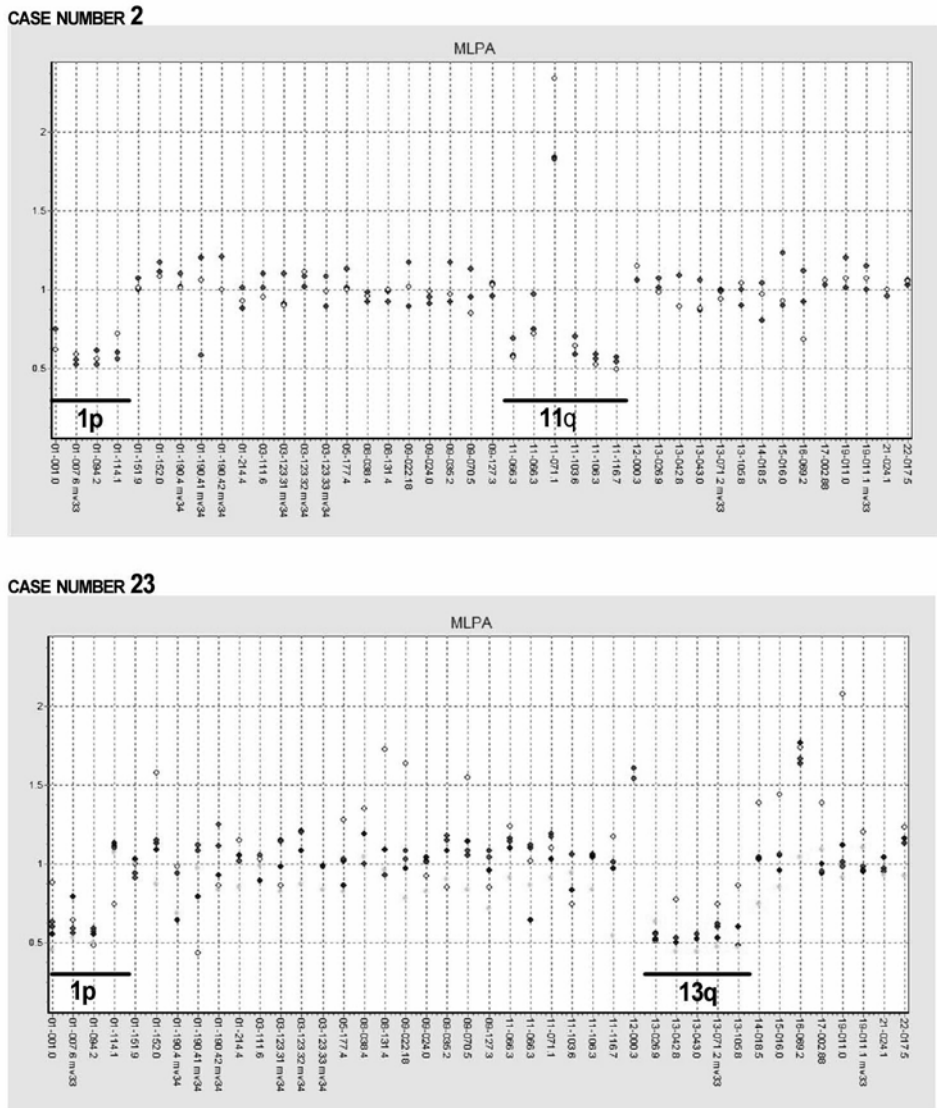
FIGURE 1 Scatter plot of 2 parathyroid carcinoma samples.
