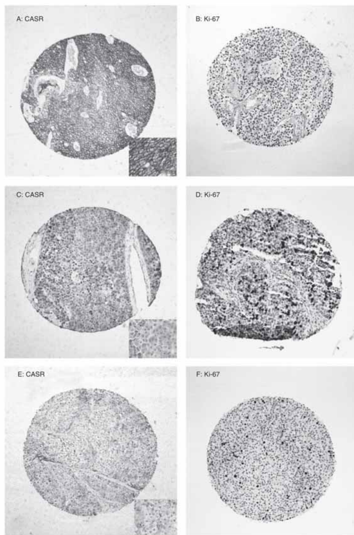
Figure 1. Immunohistochemical staining of a 5 \mu m section from a tissue micro-array showing the immunophenotype of three different parathyroid carcinomas: one (A, B) shows membranous staining from CASR (A) and no Ki-67 positivity (B); the second (C, D) shows no staining for CASR and strong Ki-67 positivity, whereas the third (E, F) shows diminished, but not absent, CASR staining, concomitant with moderate overexpression ( \geq 5\% ) of Ki-67 (magnification \times 100 ; inserts \times 200 )
