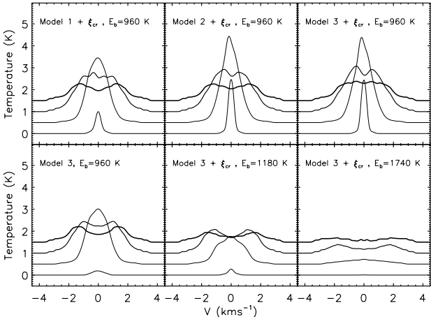
Figure 5.14: Similar to Fig. 5.13 but for C 18 O 3–2.
