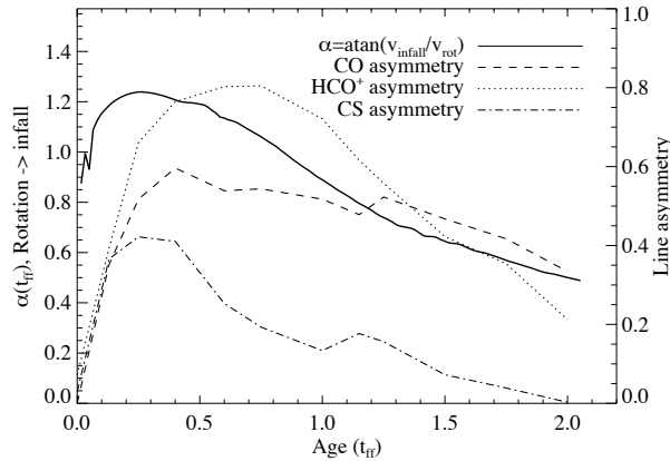
Figure 3.7: The averaged \alpha from the hydrodynamical simulation plotted against free-fall time (thick solid line). The punctured lines show the dimensionless asymmetry of the single-dish spectral lines as a function of time.
