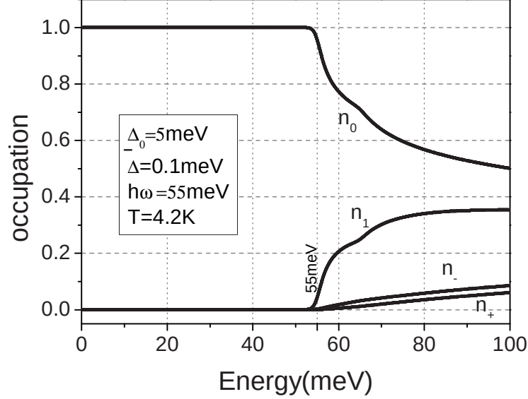
Figure 7.4: Occupation numbers of states \Psi_0 , \Psi_1 , \Psi_- and \Psi_+ as a function of the bias voltage. The system is stable in the ground state \Psi_0 until the excess energy of the electrons reaches the threshold of \hbar\omega .
