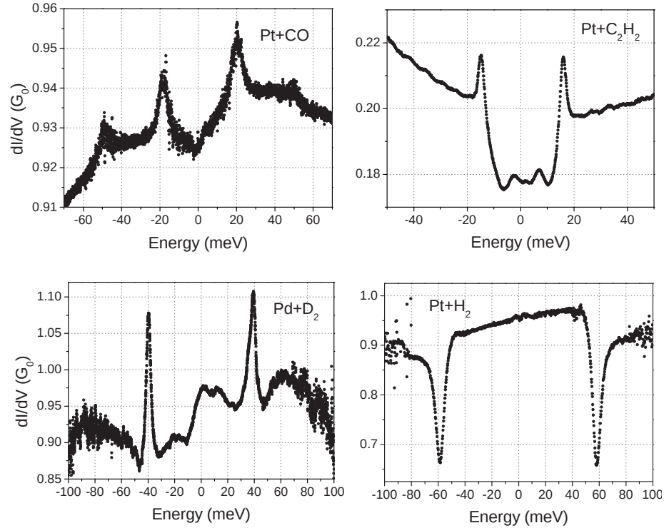
Figure 7.1: Examples of anomalous differential conductance curves as a function of the voltage. Presented curves are a small selection of curves with peaks and dips at the positions where in normal PCS spectra one finds a signature of vibration excitations.
