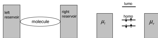
Figure 1.1: Schematic drawing of a molecular contact. The figure on the left presents the schematic picture of a molecule situated in between the electrodes and the figure on the right presents the molecule in the form of energy levels (molecular orbitals).
