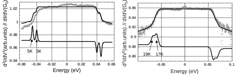
Figure 4.2: left: dI/dV curve measured on a D_2 bridge where the two steps correspond to a mode with lifted degeneracy. The temperature obtained here is around 5K for both steps at energies 40meV and 45.6meV. right: An example of a dI/dV measurement on H_2 where the large width may be partially explained by the overlap of different excitations. The temperatures obtained from the fit are 17K and 19K for vibrations centered at around 60meV and 68meV respectively. The fits have been optimized for the positive bias side.
