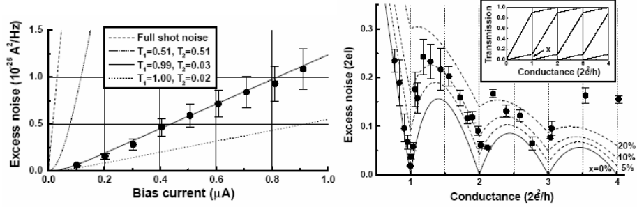
Figure 3.3: The right graph shows the shot noise measured on 27 different contacts, at 4.2K and bias current of 0.9\mu\text{A} . In the tunnelling limit, shot noise approaches the full poissonian value, while for G = nG_0 it is strongly suppressed. The left graph shows the shot noise measured for a fixed contact with G = 1.02G_0 with different bias currents and theoretical fits for a different partial transmissions of the channels contributing to the conductance. After ref. (7).
