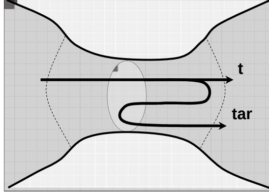
Figure 1.13: Two possible paths for electron propagation that give rise to conductance fluctuations. If the contact is partially transmitting, electrons will pass through the contact with the probability amplitude t . There is a small probability that the wave gets reflected back on defects close to the contact, resulting in a probability amplitude for electrons to return to the contact where they can be scattered back again. The path with the probability amplitude tar represents the sum over all possible scattering paths within the electron coherence length. The interference between two indicated partial waves produces the conductance fluctuations. There is a similar contribution from the waves scattering at the left of the contact.
