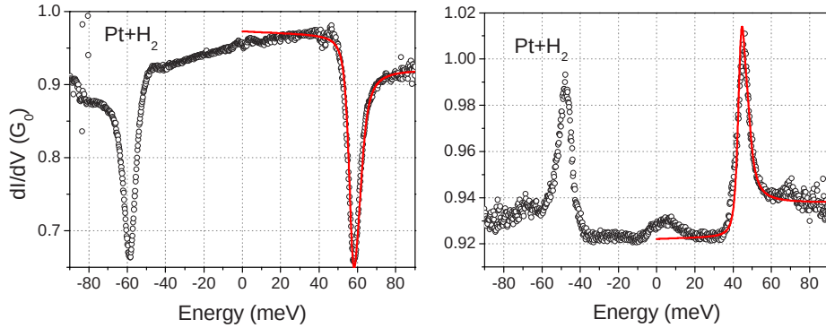
Figure 7.7: Dots represent experimental measurements of dI/dV as a function of bias and the line is a fit obtained by the vTLF model. The fitting parameters are: left panel- ( \Delta_0=1\text{meV} , \Delta=0.1\text{meV} , \hbar\omega=58.5\text{meV} , \sigma_0=0.98G_0 , \sigma_1=0.86G_0 , T=8.5\text{K} ) and right panel- ( \Delta_0=1\text{meV} , \Delta=0.3\text{meV} , \hbar\omega=45\text{meV} , \sigma_0=0.921G_0 , \sigma_1=0.955G_0 , T=7\text{K} ).
