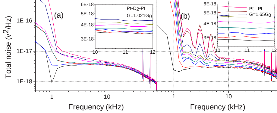
Figure 3.7: Noise as a function of the bias current for: a) \text{Pt-D}_2\text{-Pt} bridge and b) pure Pt single atom contact. The insets show the reduced range 10-12 kHz on an expanded scale. The bias current is increasing from 0 (thermal noise spectra) to 0.8\mu\text{A} . After each current adjustment, the contact is verified to remain unchanged by a dI/dV measurement.
