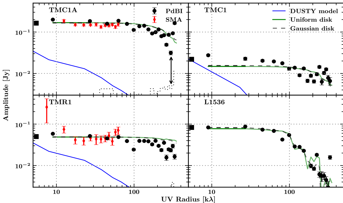
Figure 5.6 — Circularly averaged 1.36 mm visibility amplitudes as function of projected baselines in k\lambda . The black circles are from this work while the red circles are from previous SMA observations at 1.1 mm (Jørgensen et al. 2009) scaled to 1.36 mm with \alpha = 2.5 . The error bars indicate the statistical errors of each bin. The blue line is the simulated continuum emission of the spherical envelope model from Kristensen et al. (2012) sampled using the observed uv points. An arrow in the first panel shows an example of the continuum excess toward TMC1A. Solid squares are the 1.36 mm single-dish flux. The zero-expectation level given in dotted line is the expected amplitude due to noise in the absence of source emission.
