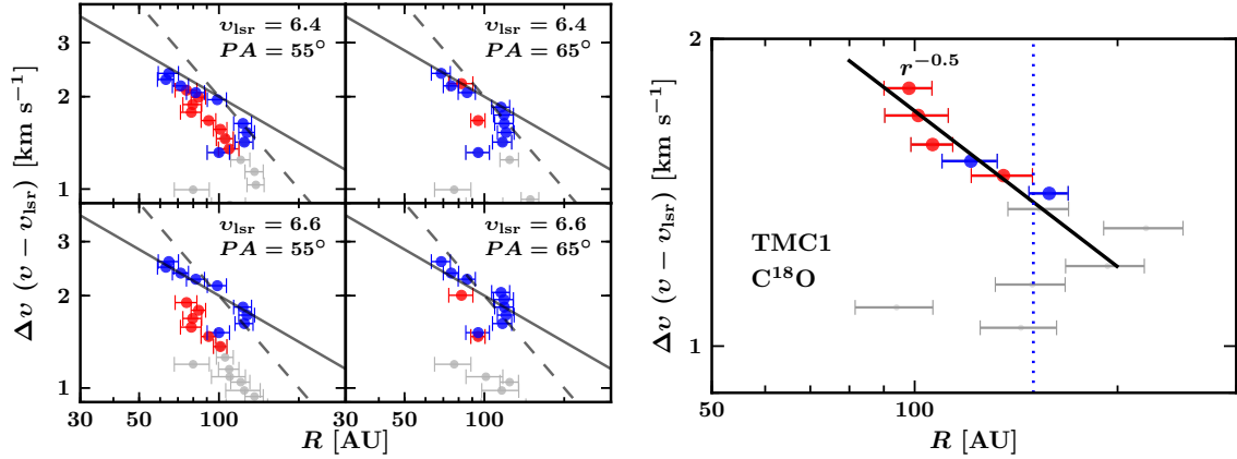
Figure 5.9 — Left: \text{C}^{18}\text{O} uv -space PV diagrams toward TMC1A with PA = 55^\circ, 65^\circ and v_{\text{lsr}} = 6.6, 6.4 km s -1 . The solid lines are the r^{-0.5} curves and dashed lines are the r^{-1} curves. The red and blue colors indicate the red- and blue-shifted components, respectively. Gray points show the rest of the peaks that were not included in the fitting. Right: \text{C}^{18}\text{O} uv -space PV diagrams toward TMC1 derived from the emission peaks. The solid line indicates the best-fit power-law slope to the peaks between 1.3–1.9 km s -1 . The vertical blue dotted lines indicate the 150 AU radius. The red and blue colors indicate the red- and blue-shifted components, respectively.
