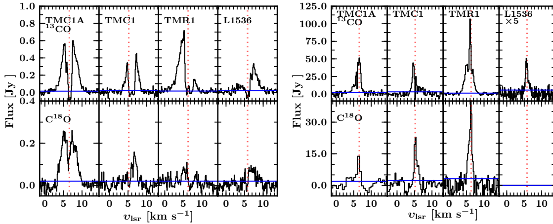
Figure 5.2 — Left : ^{13}\text{CO} (top) and \text{C}^{18}\text{O} 2–1 (bottom) spectra integrated within a 1'' box around the continuum position. Right : Single-dish spectra of ^{13}\text{CO} 3–2 (except for L1536, which is ^{13}\text{CO} 2–1) and \text{C}^{18}\text{O} 2–1. The vertical red dotted lines indicate the systemic velocities of each source derived from single dish \text{C}^{18}\text{O} and \text{C}^{17}\text{O} data (Yıldız et al. 2013). The horizontal blue lines indicate the spectral \sigma_{\text{rms}} .
