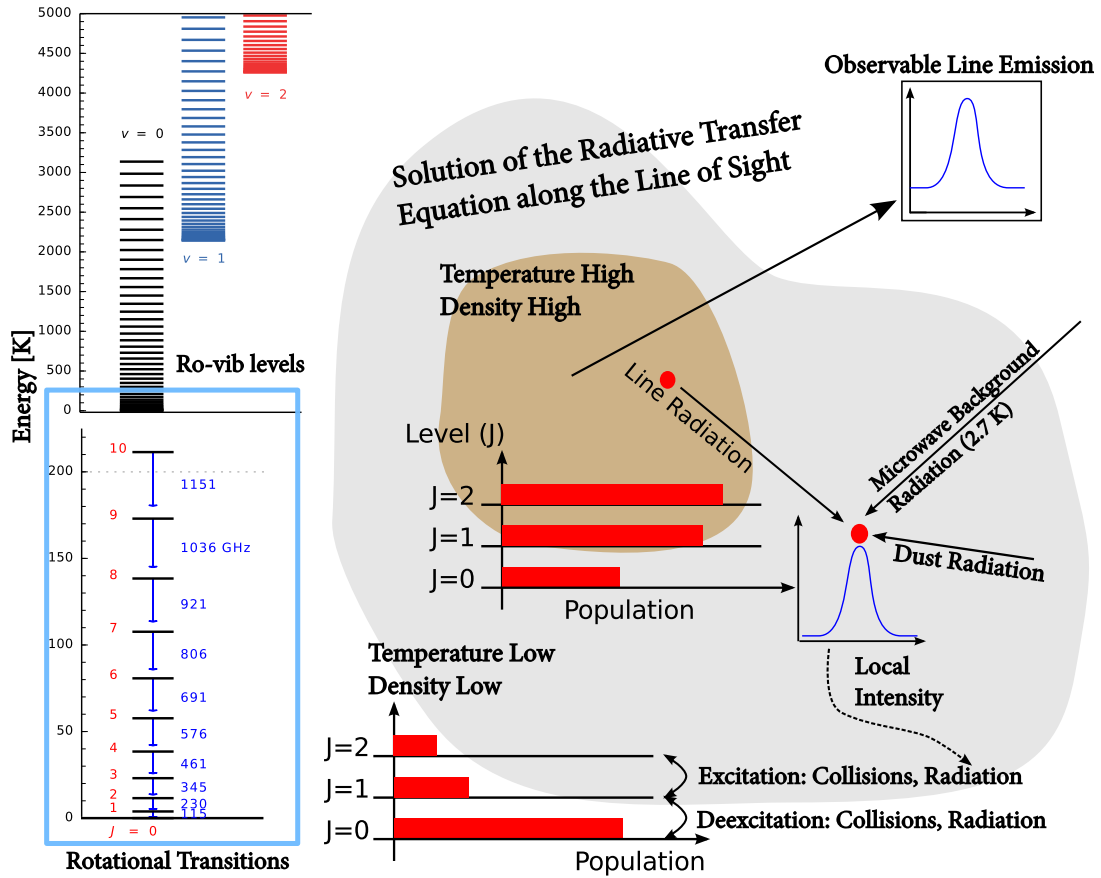
Figure 1.2 — Top left: The vibrational and rotational levels of ^{12}\text{CO} up to v = 2 and J = 40 . Bottom left: A zoom in of the rotational transitions up to J_u = 10 . A cartoon depicting the molecular line excitation and radiation propagation from an envelope to the observed line profile. The low J levels are populated in the low density and low temperature regimes while higher rotational levels are populated in dense warm gas. The excitation of molecular levels include collisions with \text{H}_2 (sometimes with \text{H} , \text{He} , and electrons) and radiation from dust, other \text{CO} molecules if sufficiently optically thick, and the cosmic microwave background at 2.7 K. Adapted from Bruderer 2010.
