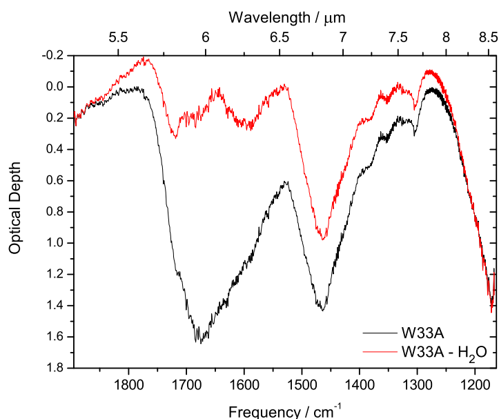
Figure 4.6 The 5.3 to 8.7\ \mu\text{m} ISO SWS spectrum of the high-mass protostar W33A plotted in optical depth together with the spectrum obtained after subtraction of the \text{H}_2\text{O} bending and librational overtone modes. The figure is adapted, with permission, from Keane et al. [2001b].
