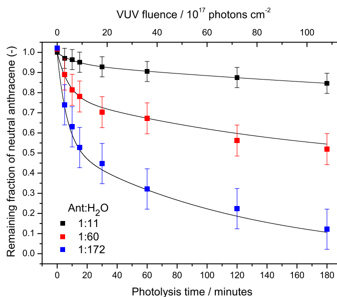
Figure 4.3 Neutral anthracene decay as a function of photolysis time (VUV fluence) and concentration for 1:11, 1:60, and 1:172 Ant:H 2 O mixtures at 15 K. Conservative errors are \pm 5 , \pm 7 , and \pm 10\% , respectively, of the initial amount of deposited neutral species. Second order exponential fits to the data (solid lines) are shown as well.
