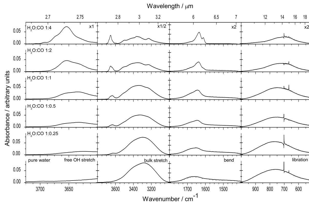
Figure 2.2 Combined spectra of the four modes for water ice for the six measured compositions (see Table 2.1), ranging from pure water ice (bottom) to a 1:4 \text{H}_2\text{O}:\text{CO} mixture (top figures). The spectra are taken at a temperature of 15 K. Note that the wavelength ranges for separate modes are different. The small structures on the libration mode are experimental artifacts.
