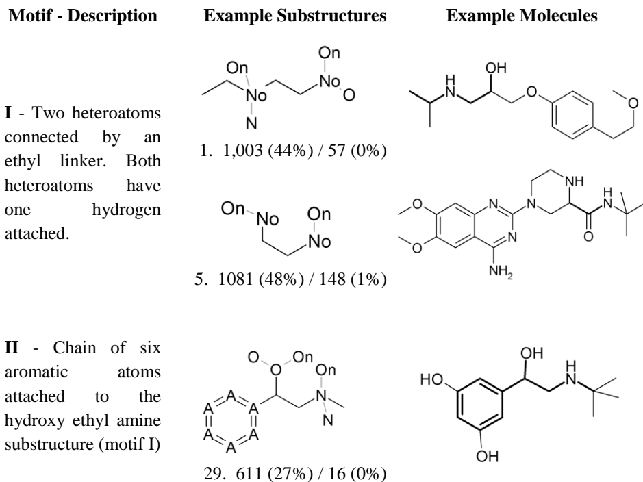
Figure 8. Common motif and example substructures for most significant substructures of the adrenoceptors ligands, in aromatic atoms and bonds representation. See legend of Figure 7 for further explanation. First example structure (for motif I) is metoprolol, a \beta_1 -adrenoceptor antagonist (beta-blocker) used to treat hypertension (taken from Klabunde et al. 51 ). The second example structure for motif I is 4-(4-amino-6,7-dimethoxyquinazolin-2-yl)-N-tert-butylpiperazine-2-carboxamide, an \alpha -adrenoceptor ligand and prazosin derivative found in GLIDA. 33 The example structure for motif II is terbutaline, a \beta_2 -adrenoceptor agonist used in the treatment of asthma.
