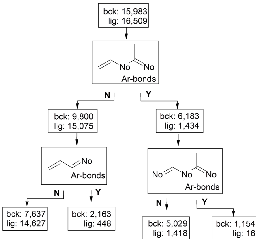
Figure 5. Hierarchical splits for the DIVERSet background compounds compared to GPCR ligands (hGPCR-lig). See legend to Figure 3 for further explanation. Here, it is particularly remarkable that the substructures all contain a double bonded heteroatom. The substructures at the top and right path match the carboxyl and ester groups, which are abundant in the DIVERSet.
