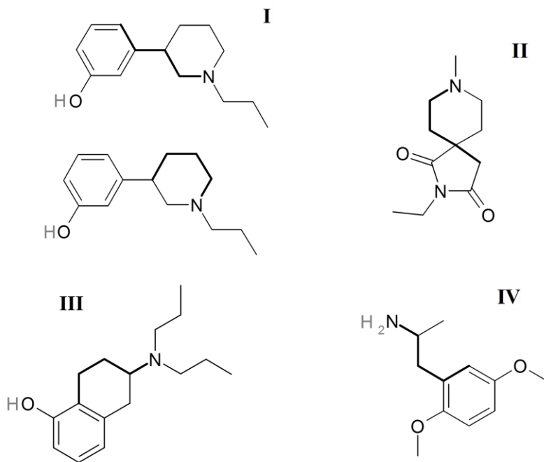
Figure 2. Example overlays on GPCR ligands of the most discriminative substructure, ‘normal’ representation. For the first ligand (I), two possible overlays are shown; multiple overlays are also possible for the ligands II and III. Note that the ‘normal’ representation uses Kekulé structures for aromatic systems and not separate types for delocalized bonds and aromatic atoms. This results in some interesting examples where the single bond of an aromatic ring is part of the aliphatic chain of the overlaid substructure, i.e. in structures I and IV.
