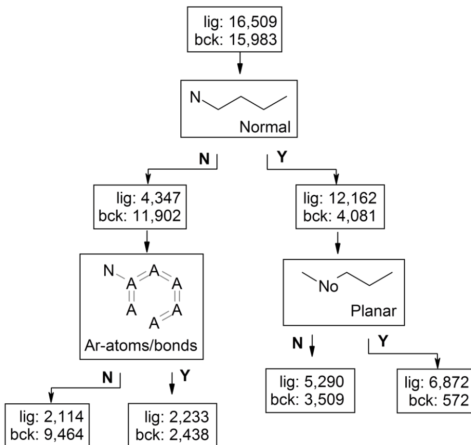
Figure 3. Hierarchical partitioning of GPCR ligands (hGPCR-lig – lig) versus background compounds (DIVERSet - bck). Ligands having the first substructure are taken out of the two sets (left path, N for ‘No’) or rather kept (right path, Y for ‘Yes’), and the process of substructure mining is repeated. Numbers given are the absolute numbers of molecules used. Most discriminative substructures in any elaborate representation are shown. The name of the representation that yielded this substructure is given at the bottom of the box surrounding the substructures.
