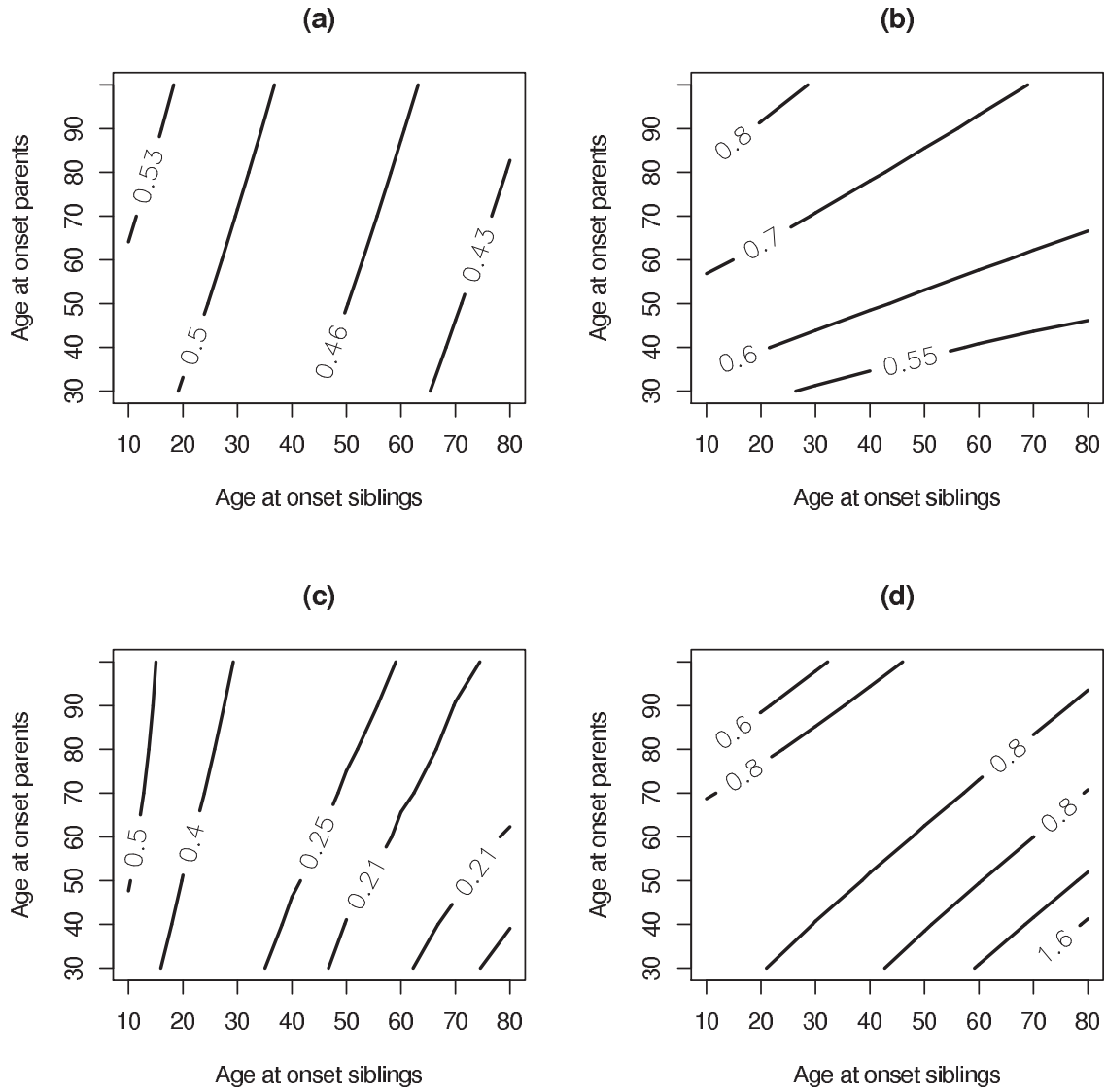
FIGURE 3.1: Weights corresponding to the gamma frailty model as a function of the age at onset of the ASP and their affected parents. Fig. 1(a): rare disease and \sigma_G^2 = 1 . Fig. 1(b): rare disease and \sigma_G^2 = 5 . Fig. 1(c): common disease and \sigma_G^2 = 1 . Fig. 1(d): common disease and \sigma_G^2 = 5 .
