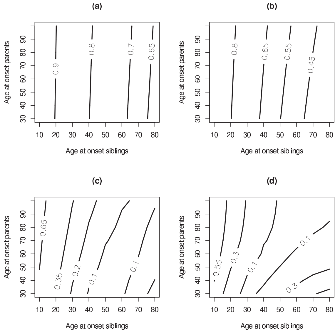
FIGURE 3.2: Weights corresponding to the log-normal model as a function of the age at onset of the ASP and their parents. Fig. 2(a): rare disease and \sigma_N^2 = \log(1 + 1) . Fig. 2(b): rare disease and \sigma_N^2 = \log(1 + 5) . Fig. 2(c): common disease and \sigma_N^2 = \log(1 + 1) . Fig. 2(d): common disease and \sigma_N^2 = \log(1 + 5) .
