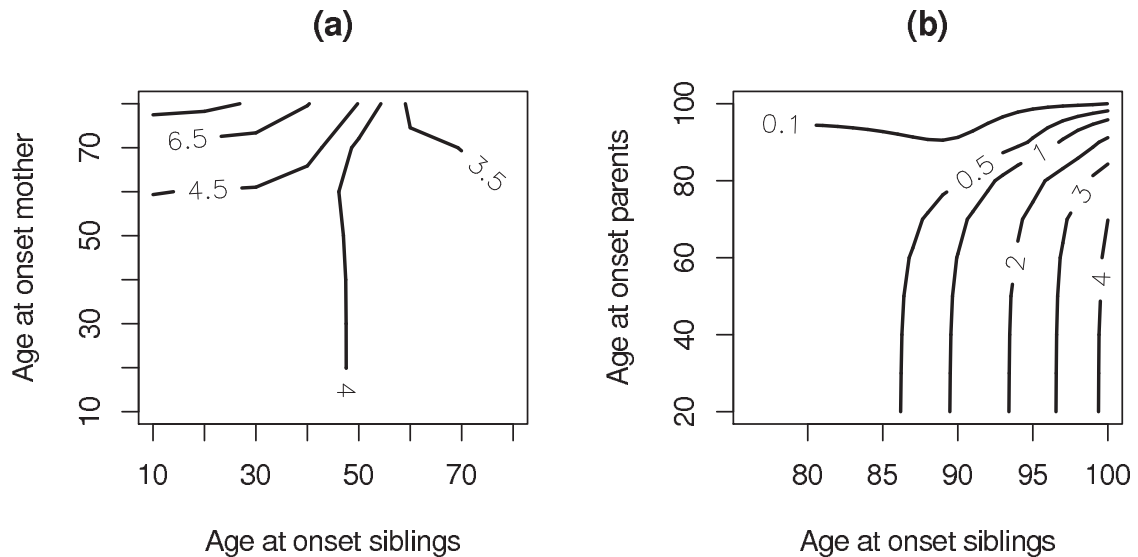
FIGURE 3.4: Weights corresponding to realistic models for breast cancer (Fig. 4(a)) and for human life span (Fig. 4(b)).
