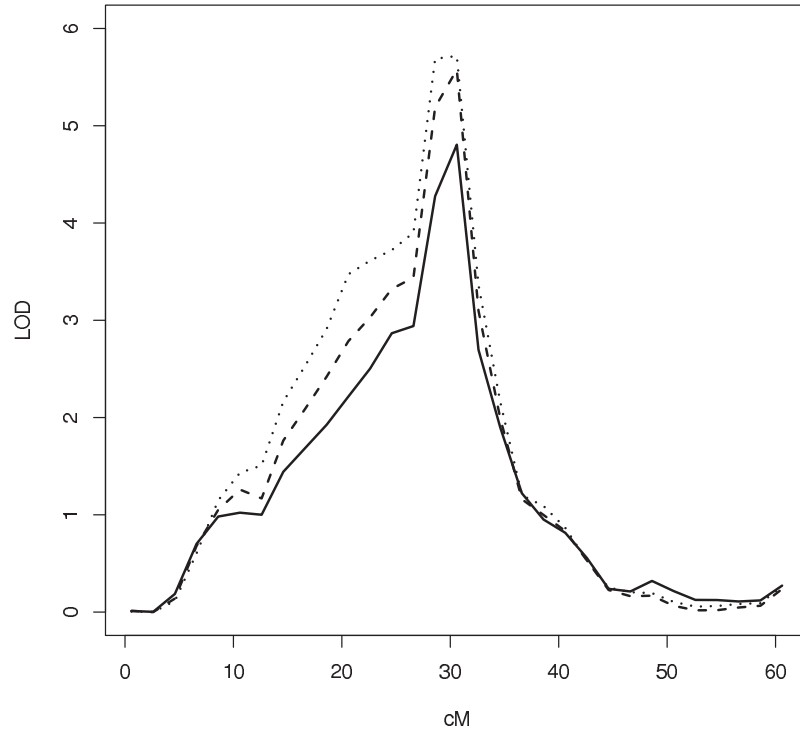
FIGURE 3.6: Genetic Linkage analysis of the GAW12 data on chromosome 6. Straight lines represents NPL method, dashed line represents NPL_G^p method, and pointed line represents NPL_N^p method.
