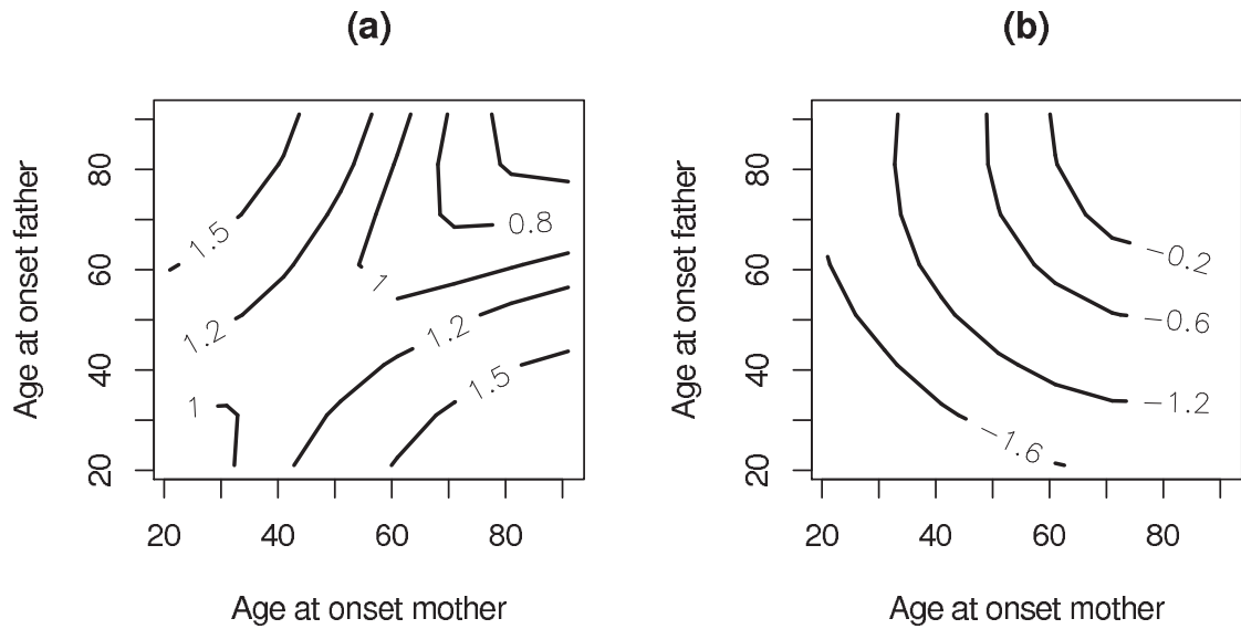
FIGURE 3.3: Weights corresponding to the gamma frailty model as functions of the age at onset of the two parents for a common disease with \sigma_G^2 = 5 . Fig. 3.3(a): early onset ASP. Fig. 3(b): discordant sibling pairs.
