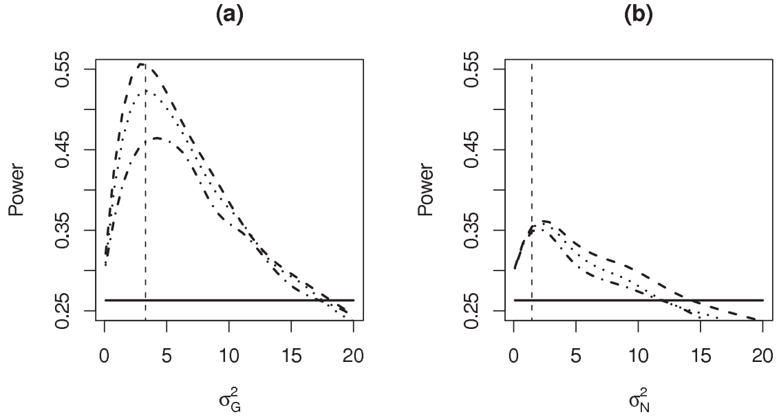
FIGURE 3.5: Power of the test statistics based on simulated data (significance level \alpha = 0.05 ). The horizontal lines represent the power of the unweighted NPL (solid line). Dashed lines, dotted lines, dashed-dotted lines represent the power of proposed NPL methods assuming a^2 = 0.25, 0.5 and 0.75 , respectively. Figure on the left (a): NPL_G^p . Figure on the right (b): NPL_N^p .
