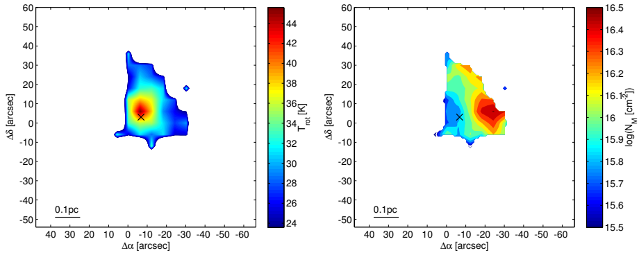
Figure 4.37: S255: Maps of CH 3 OH rotation temperature and column density.
