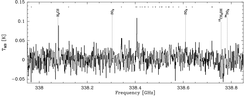
Figure 4.18: G24.541+00.312 : Spectrum of the maser position. The tick marks at the top indicate the frequencies of the methanol lines.
