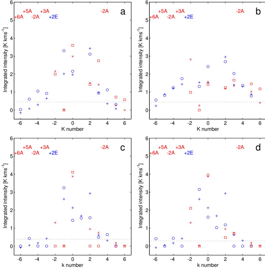
Figure 3.7: Plots of the integrated intensity for different CH 3 OH 7_K \rightarrow 6_K transitions and the best \chi^2 model values. In the panels the observed flux (open symbols) is plotted, as well as the non-LTE model values (plusses and crosses). Also indicated is the 3\sigma detection limit. Circles and plusses (blue) are used for E-type lines and squares and crosses (red) for A-type. Labels on the top identify blended lines, for which the combined flux and model value are displayed. The K=+1 line which is blended with an SO 2 was not included in the analysis for the centre region components (top panels). The parameters of the fits are listed in Table 3.3. a : main, -10.5 \text{ km s}^{-1} velocity component at the "Centre" position with beam dilution factor of 1, b : red-shifted, -5.2 \text{ km s}^{-1} velocity component at "Centre" with a beam dilution factor of 50, c : the "NE Outflow" and d : "Envelope".
