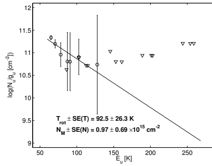
Figure 4.21: G40.62–0.14 : Rotation diagram of \text{CH}_3\text{OH} at the position of the maser.
