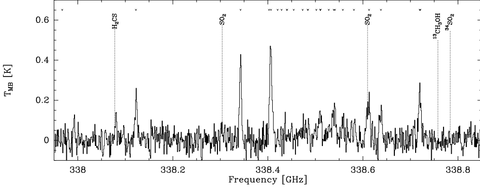
Figure 4.19: G40.62–0.14 : Spectrum of the maser position.
