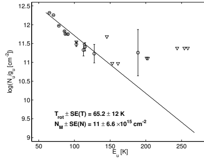
Figure 4.3: AFGL 5142: Rotation diagram of \text{CH}_3\text{OH} for the position of the maser.
