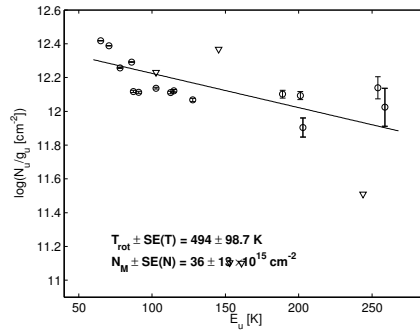
Figure 4.40: W3(OH): Rotation diagram of \text{CH}_3\text{OH} for the position of the maser.
