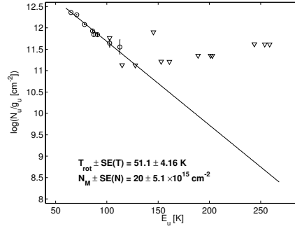
Figure 4.11: G23.207–00.377 : Rotation diagram of CH 3 OH for the maser position.
