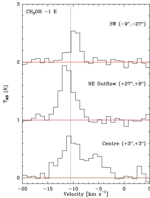
Figure 3.2: Velocity profiles of the -1 E line at three positions. Although the profiles are Gaussian in the outflow, there is a clear shift in the velocity. At the “Centre” position there are clearly two velocity components. The dotted line is taken to be the system velocity, corresponding to the velocity of the dominant component at the “Centre” position.
