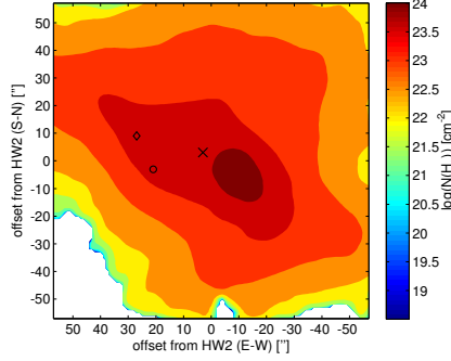
Figure 3.8: H_2 column densities derived from the SCUBA dust continuum for a constant dust temperature of 30 K.
