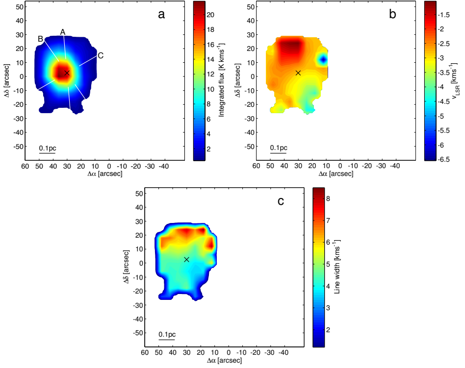
Figure 4.2: Integrated intensity (a), central velocity (b) and FWHM width (c) of the \text{CH}_3\text{OH} 7(-1) \rightarrow 6(-1) E line observed toward AFGL 5142. The black cross marks the position of the 6.7 GHz maser and the outflow directions A, B, and C (Zhang et al. 2007) are indicated by the white lines.
