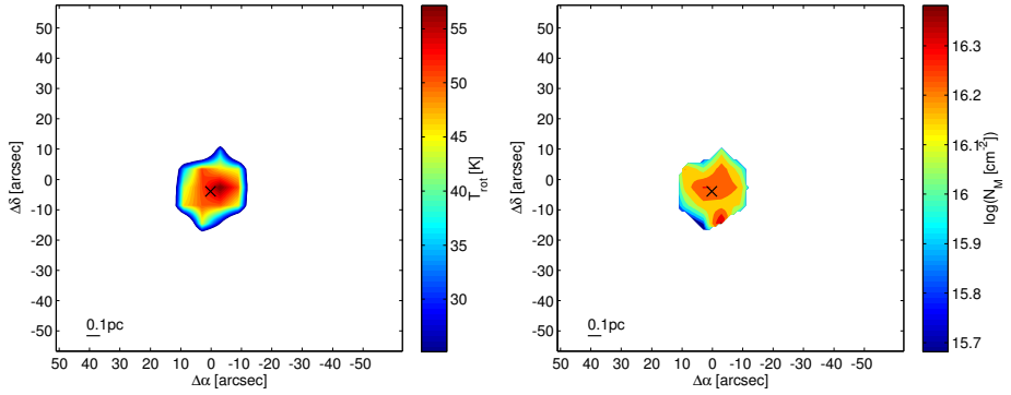
Figure 4.12: G23.207–00.377 : Maps of CH 3 OH rotation temperature and column density.
