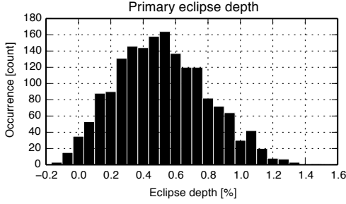
Figure 5.4: All long cadence transit depths obtained from scaling the best-fitting model to SAP_FLUX data. Here we plot the depth at the minimum of those scaled models. The few negative eclipse depths are due to noise in the data.
