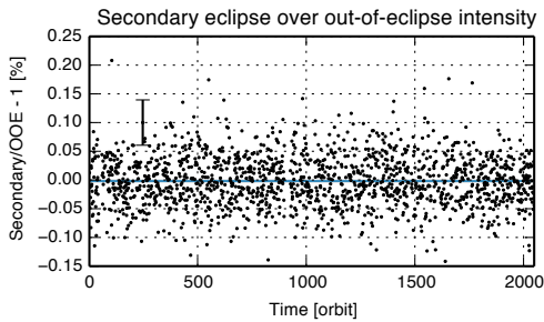
Figure 5.10: Long cadence flux during the secondary eclipse divided by flux during out-of-eclipse periods as a function of orbit. The weighted-average three-sigma upper limit is 4.9 \times 10^{-5} . The black error bar is the mean error of the individual data points.
