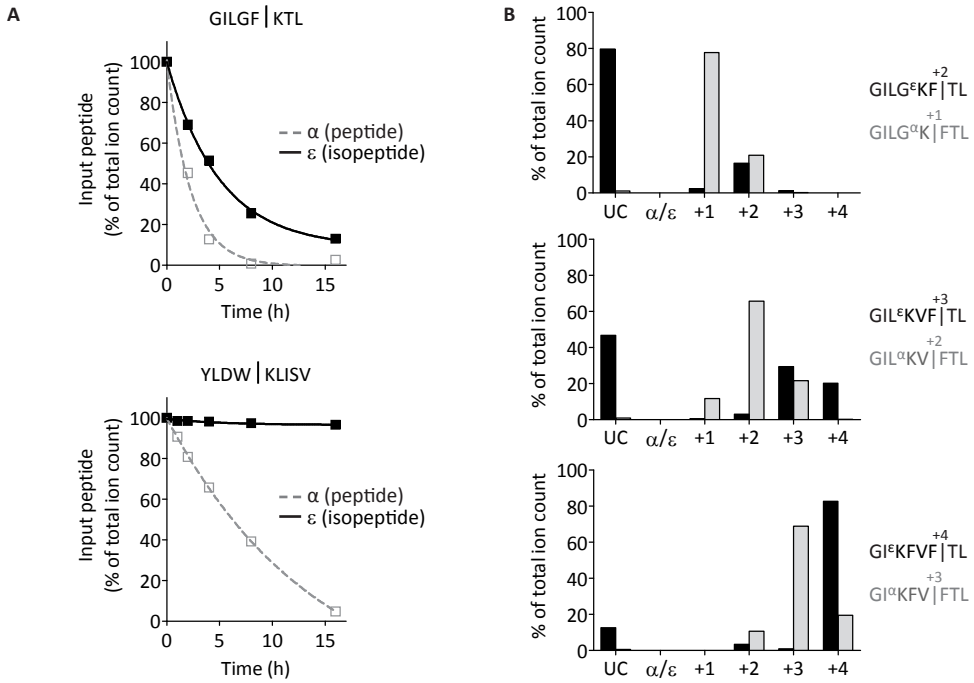
Figure 4 | Isopeptides show enhanced stability towards proteasomal degradation. A) Degradation of GILGF \alpha/\epsilon KTL and YLDW \alpha/\epsilon KLISV by the proteasome as a function of time. The amounts of input peptides and degradation products were quantified using LC-MS. The site of cleavage and the location of the lysine N \alpha - or N \epsilon -linkage is indicated with a vertical line. B) Proteasomal degradation patterns of the indicated peptides. The amounts of input peptides and degradation products were quantified using LC-MS after incubation with proteasome for 16 h. Black bars indicate isopeptides and corresponding degradation products, grey bars indicate normal peptides and corresponding degradation products. The main site of cleavage is indicated with a vertical line. The location of the lysine N \alpha - or N \epsilon -linkage is indicated with \alpha or \epsilon . Cleavage products are indicated by the site of cleavage relative to the lysine N \alpha - or N \epsilon -linkage. UC: uncleaved input peptide.
