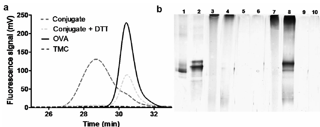
Figure 4: (a) GPC chromatograms based on fluorescence detection (ex 295 nm, em 340 nm) of TMC-OVA conjugate (Conjugate), reduced TMC-OVA conjugate (Conjugate + DTT), OVA, and TMC. (b) SDS-PAGE under reducing (even lanes) and non-reducing (odd lanes) conditions of OVA (lane 1,2), TMC (lane 3,4), TMC-OVA conjugate fractions 25-27 min (lane 5,6), 27-29.5 min (lane 7,8) and 29.5-32 min (lane 9,10).
