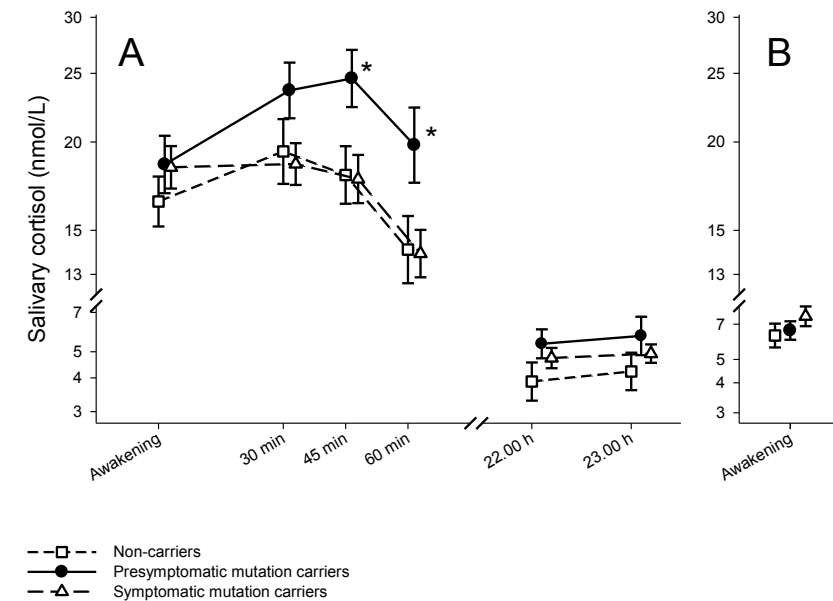
Figure 1. Salivary cortisol concentrations of the day curve and post-DST
