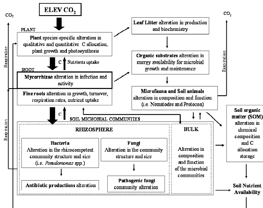
Fig. 1: Conceptual model which describes the response of dominant plant species to elevated atmospheric CO 2 . The increased photosynthetically C allocation is initially directed mainly to mycorrhizae and root tissue. Mycorrhizae are translocating C into the soil microbial communities, thereby changing the structure, size and activity of the rhizosphere microbial community (Bacteria and Fungi) to a larger extent than the community of the bulk soil. Soil microbial communities subsequently affect food web interactions and mediate the ecosystem feedbacks that regulate the cycling of C and N.
