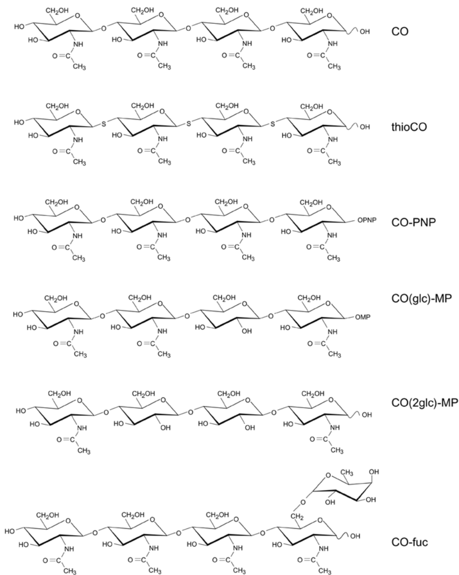
Figure 2. Structures of CO derivatives. CO: chitin oligosaccharide; thioCO: CO in which the oxygen atoms of the \beta(1\rightarrow4) linkages are substituted by sulfur atoms; CO-PNP: CO with PNP modification at C1 position; CO(glc)-MP and CO(2glc)-MP: one or two GlcNAc residues are replaced by glucose, respectively, and with MP modification at C1 position; CO-fuc: fucosylated CO.
