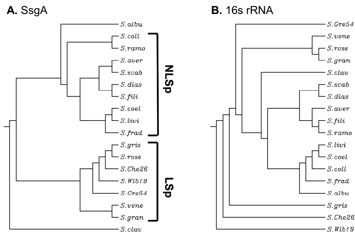
Figure 7. Phylogenetic tree of SsgA proteins and 16S rRNA sequences. Phylogenetic trees are shown for SsgA (A) and 16S rRNA (B) from 18 Streptomyces strains (see Results section). Two major branches of SsgA proteins are indicated, namely: SsgA orthologues from strains that produce spores in liquid-culture (LSp branch), SsgA orthologues from strains that produce dense mycelium clumps and no spores in liquid-culture (NLSp branch). SsgA and 16S rRNA were labelled by their strain of origin, for sequence labels see "Computer analysis" in "Materials and Methods"
