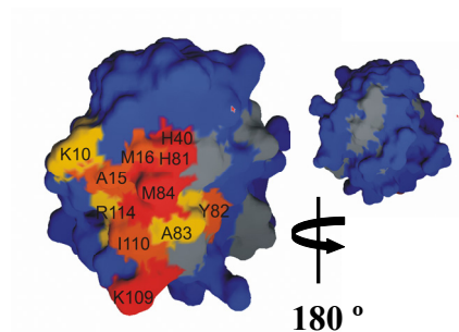
d) PAZ Cu I : NiR Cu I-T2D (cross saturation transfer method)
