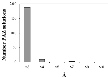
Distance between Gly200 (NiR) and PAZ
