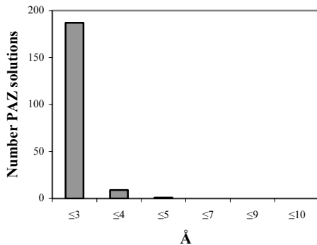
Distance between Gly200 (NiR) and PAZ
