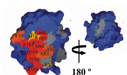
c) PAZ Zn II : NiR Cu II-Cu II (direct titration)
