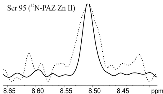
Figure 3.6: Cross-section through the ^1\text{H} resonance of Ser95 of ^{15}\text{N} -PAZ Zn II. The solid line represents the signal of the free protein. The signal with the dotted line was taken when the ratio NiR Cu I-T2D / PAZ Zn II is 0.15. The line width at half-height is 22 Hz and 41 Hz, respectively.
