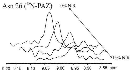
Figure 3.7: Cross-section along the F_2 dimension through the ^1\text{H} resonance of Asn26 ( ^{15}\text{N} -PAZ Zn II). The figure shows the decrease in the intensity of the amide signal upon addition of NiR Cu I-T2D. ^{15}\text{N} -PAZ Zn II amide signal becomes undetectable at the experimental conditions when 0.2 mol.eq. of NiR Cu I-T2D subunit is added
