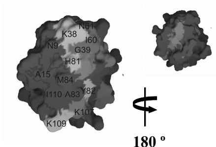
Figure 6.3: Mapping of the \Delta\delta_{avg} on the surface of PAZ (front side on the left and back side on the right) for the complexes a) NiR Cu I-T2D : ^{15}\text{N} -PAZ Cu I at a ratio of 1.7 in the inverse titration; b) NiR Cu I-T2D : ^{15}\text{N} -PAZ Zn II at a ratio 0.15 in the direct titration; c) NiR Cu II-Cu II : ^{15}\text{N} -PAZ Zn II at a ratio of 0.10 in the direct titration and d) map obtained with cross saturation transfer for complex formation between NiR Cu I-T2D and ^{15}\text{N} -PAZ Cu I at a ratio of 0.7. Residues are colour-coded according with the horizontal line in Figure 6.2a, b and c (for Figure 6.3a, b and c respectively). In figure 6.3d the colour code according to the classification shown in Figure 5.2 in Chapter 5 has been used. (For a color picture see Appendix).
