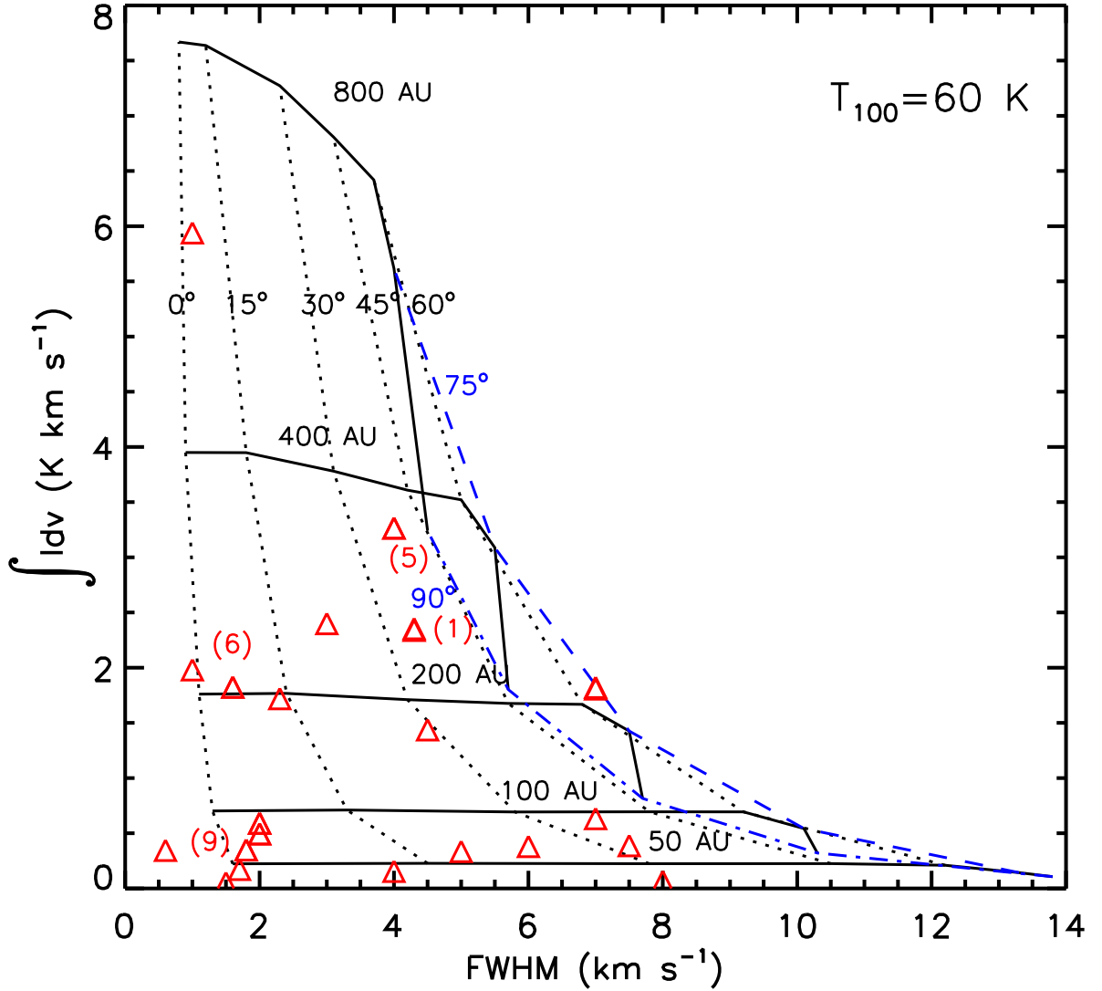
Figure 5.3: Integrated intensity of the modelled ^{12}\text{CO} J=3-2 line emission, plotted versus the FWHM, for M_{\text{star}}=2.0 M_{\odot} and M_{\text{disc}}=0.01 M_{\odot} . The figure shows the results of the parametric disc models with T_{100}=60 K. The full black lines connect the results of models at a constant disc outer radius, the value of which is labeled. The dotted and the dashed lines connect the results for a constant inclination, also labeled. The triangles are the observed values, from Dent et al. (2005) and this work, with the observed integrated line intensities scaled as \int IdV \times (d/140 \text{ pc})^2 . Some of the sources from Table 5.1 are labeled by number.
