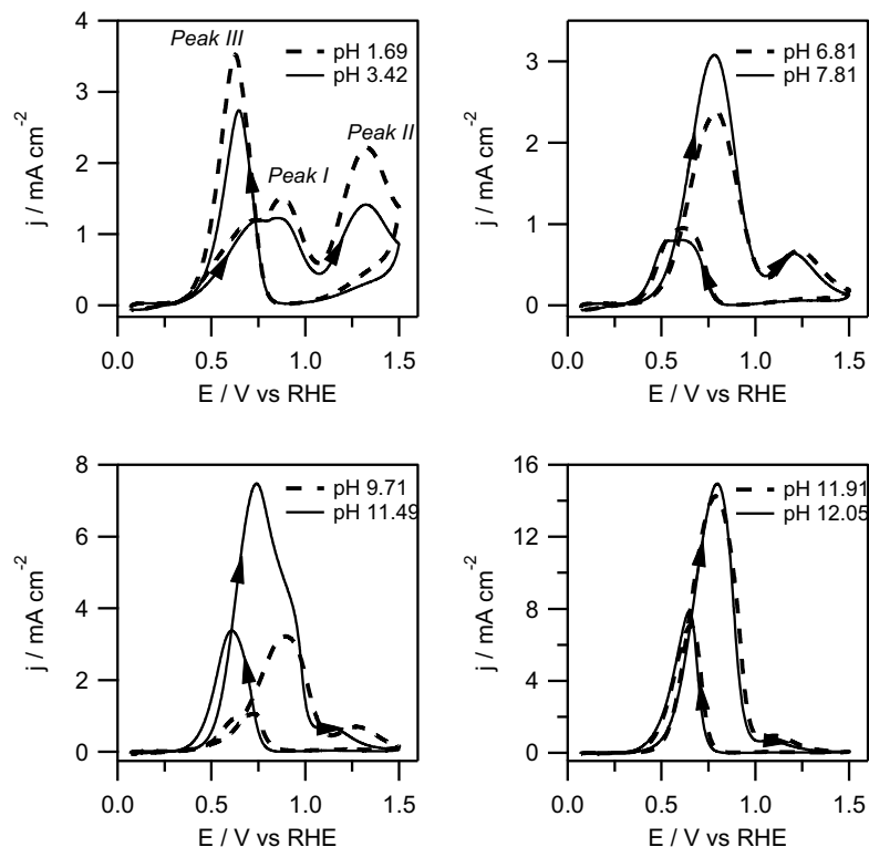
Figure 7.6: Cyclic voltammograms for the oxidation of 0.5 M ethanol in 0.1 M phosphate buffers (ca. pH 1 - 12) on polycrystalline platinum. The voltammograms are recorded at 50 \text{mV s}^{-1} . The arrows indicate the scan directions.
