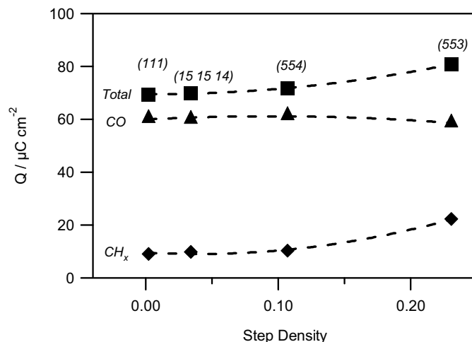
Figure 3.8: Structure sensitivity of ethanol adsorbate stripping in 0.1 M HClO 4 as implied by the amount of charge in the H_{UPD} region that is inhibited by the adsorbates. Triangles denote oxidizable species, while diamonds reducible species. Squares indicate the sum of the oxidizable and reducible species. The dashed lines are drawn to guide the eye.
