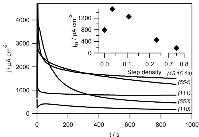
Figure 3.11: Current-time transients of the oxidation of 0.5 M acetaldehyde in 0.1 M HClO 4 . The step potential was 0.7 V. The inset shows the current density after 15 minutes as a function of step density.
