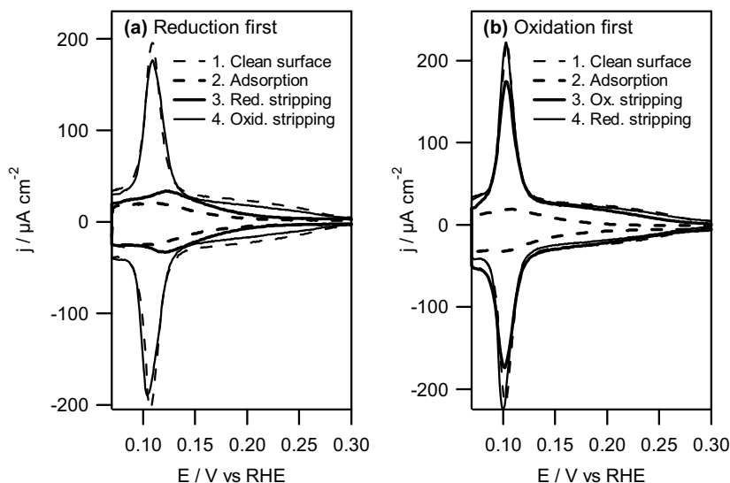
Figure 3.5: Typical voltammetric profiles of the H_{UPD} region at various stages of the ethanol adsorbate stripping experiments on Pt (553) in 0.5 M H_2SO_4 . After initial adsorption at 0.4 V, the surface was subjected to (a) reductive stripping first followed by oxidative stripping, and (b) oxidative stripping first followed by reductive stripping. The voltammograms were recorded at 50 \text{ mV s}^{-1} .
