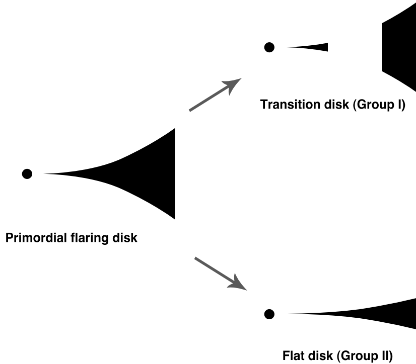
Figure 3.14: Sketch of an evolutionary scenario for disk evolution in Herbig Ae/Be objects (after Currie 2010). Both groups have evolved from a common ancestor (i.e. primordial, possibly embedded, flaring disk structure). In transitional group I objects, gap formation proceeds the collapse of the outer disk. In group II objects, grain growth and dust settling have flattened the outer disk.
