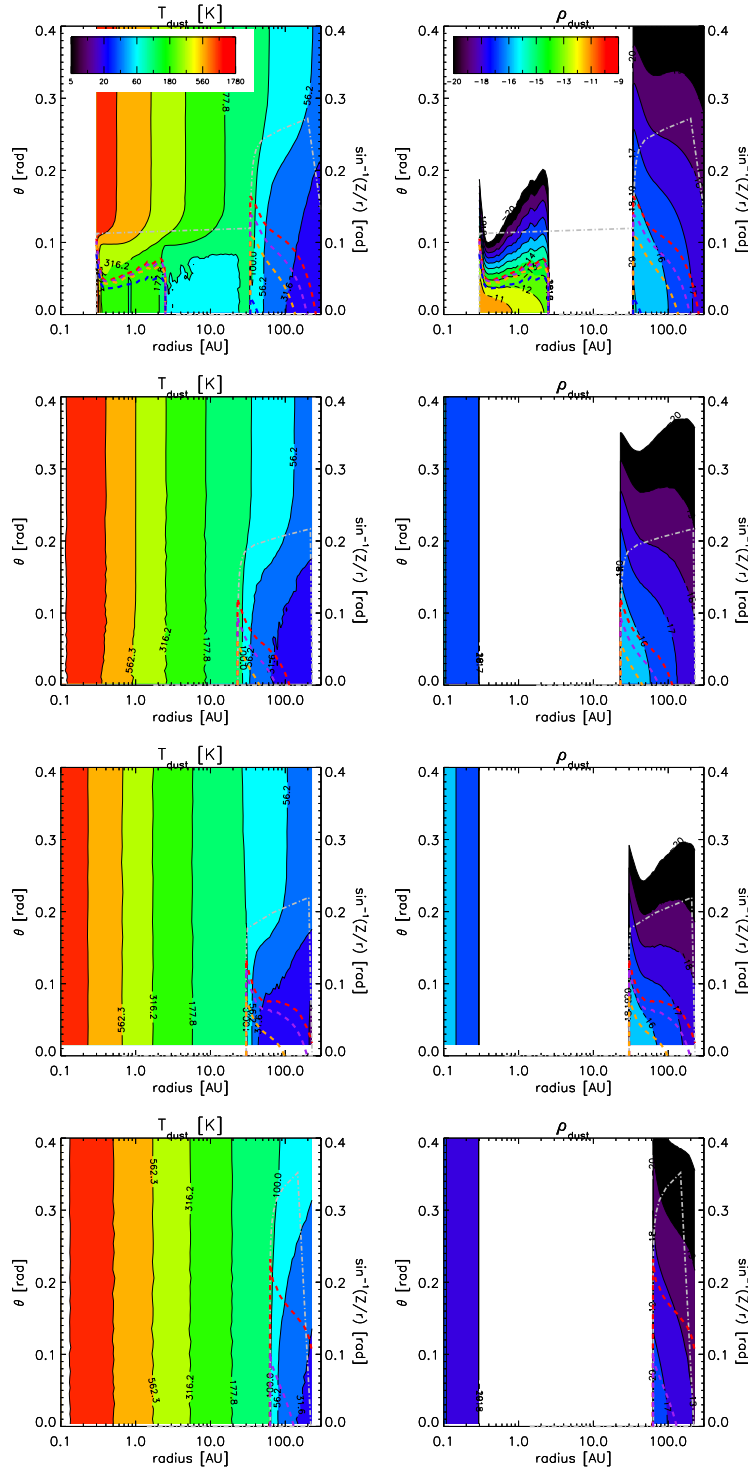
Figure 3.7: Left: radial temperature distribution (K). Right: density ( \text{g cm}^3 ) structures of the disks. Top to bottom: HD 97048, HD 169142, HD 135344 B and Oph IRS 48. The dashed lines represent the \tau = 1 surfaces as seen perpendicular from the disk. From top to bottom, the colors are red, purple, orange, and blue and represent the wavelengths 1, 20, 70, and 1000 \mu\text{m} . The gray dot-dashed line shows the \tau = 1 surface in radial direction in scattered light ( \lambda = 0.5 \mu\text{m} ). Note that HD 97048 has a thick inner disk, and therefore the radial \tau = 1 surface starts at the rim of the inner disk.
