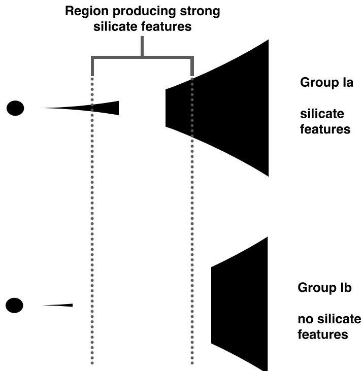
Figure 3.13: Sketch showing the region where (sub-) micron-sized silicate grains have a temperature ( T \sim 200\text{--}400\text{ K} ) where they produce strong silicate features. Transitional group Ia sources (top) show silicate features, because the inner disk and/or the outer disk wall have a sufficient amount of silicate dust in this region. In the group Ib objects of our sample (bottom), the silicate dust is severely depleted in this region, and thus, no silicate features are produced.
