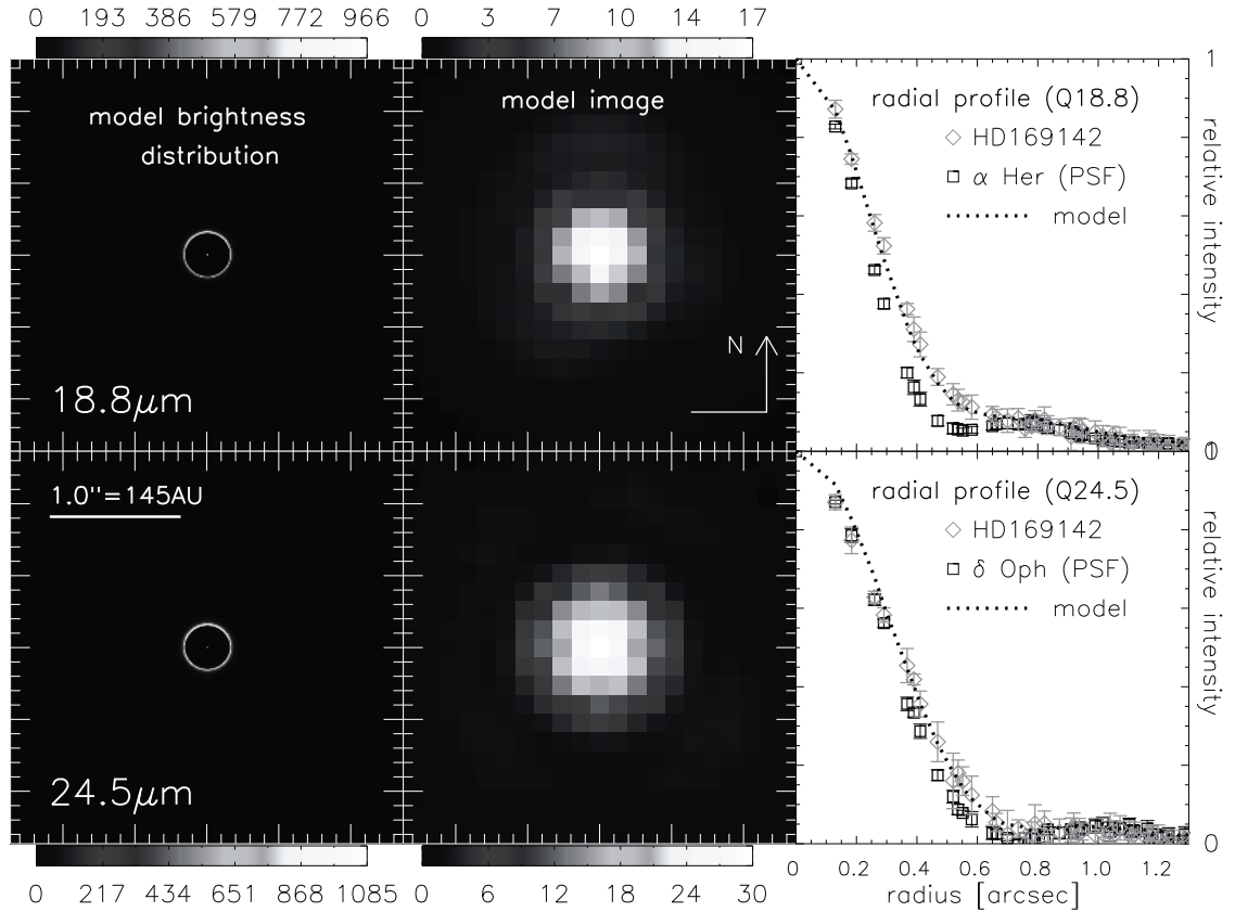
Figure 2.2: Left and middle panels are model brightness distribution of final model and model image after convolved by Subaru/COMICS PSF (middle), respectively, shown in Jy/arcsec 2 . Right panels represents the peak-normalized azimuthally-averaged radial brightness profiles relative to the centroid of the image (right). Top panels are in the Q18.8 and the bottom panels are in the Q24.5 filters. In the radial profile plots (right), the observation of HD 169142 is shown by the diamonds, and the corresponding PSF of the calibrators is shown by the squares. The final model convolved with the PSF is shown by the dotted line.
