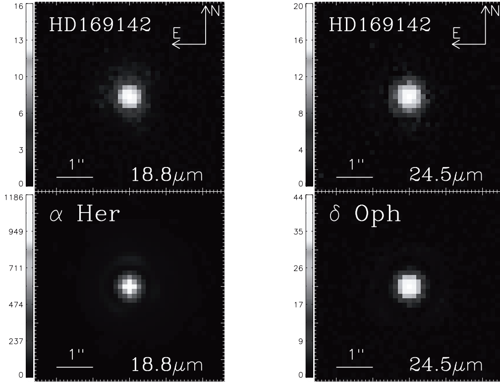
Figure 2.1: Shift-and-added image of HD 169142 (top) and PSF star (bottom) at 18.8 and 24.5 \mu\text{m} . Brightness unit is in \text{Jy/arcsec}^2 and scaled from 0 to the peak value in the image. North is up and the east is to the left
