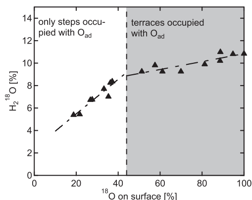
Figure 6.7 Isotopic partitioning of \text{H}_2^{18}\text{O} vs. the amount of pre-adsorbed ^{18}\text{O}_2 when Pt(553) is covered with \sim 1 \text{ ML H}_2^{16}\text{O} . The dashed line marks the point where the (111) terrace starts to become occupied with ^{18}\text{O}_{\text{ad}} .
