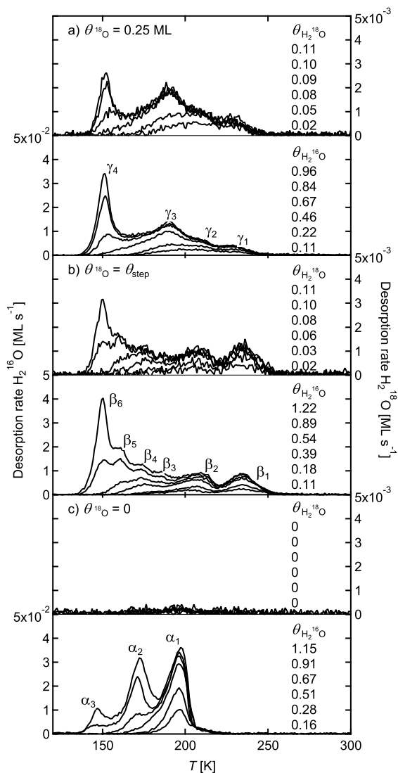
Figure 6.2 TPD spectra of H 2 16 O (left axis) and H 2 18 O (right axis) dosed on a) Pt(553) with \theta_{^{18}\text{O}} = 0.25 ML, b) \theta_{^{18}\text{O}} = \theta_{\text{step}} , and c) \theta_{^{18}\text{O}} = 0 .
