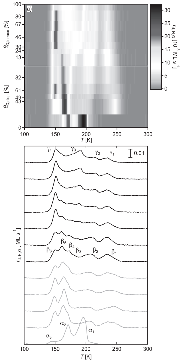
Figure 6.5 TPD spectra of \sim 1 \text{ ML H}_2\text{O} desorbing from Pt(553) with varying \text{O}_{\text{ad}} pre-coverages of the steps sites (bottom half) and the full step and part of the terrace sites (top half).
