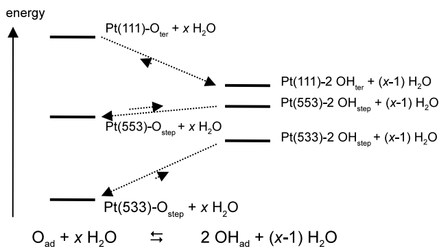
Figure 4.4 Schematic representation of the energy levels for the co-adsorption of O ad and H 2 O on Pt(111), Pt(553), and Pt(533).
