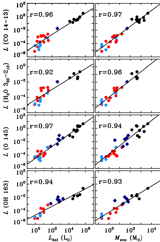
Figure 3.4 – Correlations of line emission with bolometric luminosity (left column) and envelope mass (right column) from top to bottom: CO 14-13, H 2 O 3 03 -2 12 , [O I] at 145 \mu m line luminosities. Low- and intermediate-mass young stellar objects emission is measured over 5 \times 5 PACS maps. Red and blue circles show Class 0 and Class I low-mass YSOs from Karska et al. (2013). Blue diamonds show intermediate-mass YSOs from Wampfler et al. (2013; O and OH lines) and from Fich et al. (2010; CO and H 2 O line). High-mass YSOs fluxes are measured in the central position and shown in black. Pearson coefficient r is given for each correlation.
