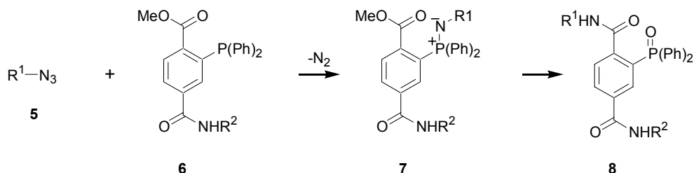
Scheme 1. Staudinger-Bertozzi ligation to connect R^1 and R^2 .
