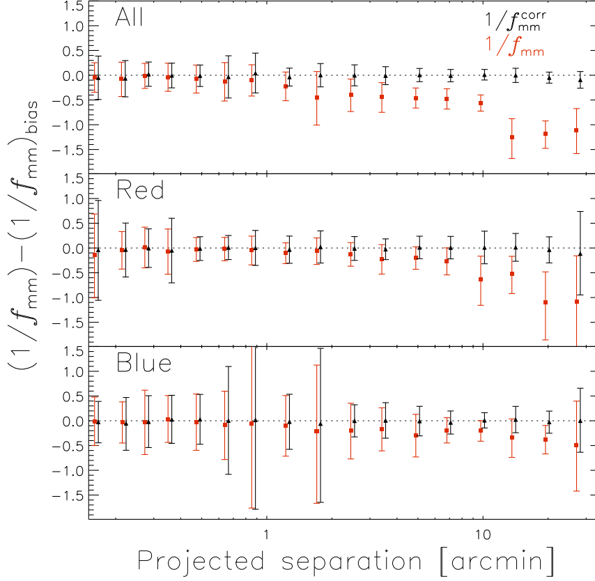
Figure 5.7: Difference between the original and the PSF biased shear ratios (1/f_{\text{mm}}^{\text{corr}}) - (1/f_{\text{mm}}^{\text{corr}})_{\text{bias}} (black triangles) and (1/f_{\text{mm}}) - (1/f_{\text{mm}})_{\text{bias}} (red squares) as a function of projected separation from the lens for the three lens samples. We find that the PSF residuals are properly removed from the corrected ratio 1/f_{\text{mm}}^{\text{corr}} , as the difference is consistent with zero on all scales. For the uncorrected ratio 1/f_{\text{mm}} , the difference is negative and decreases with projected separation. This result shows that the cross term effectively removes PSF residuals in the shear ratio estimators.
