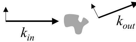
Figure 1: The main effect of a scattering event is to change the direction of propagation of light. The polarization direction is indicated by the small transverse arrow.
