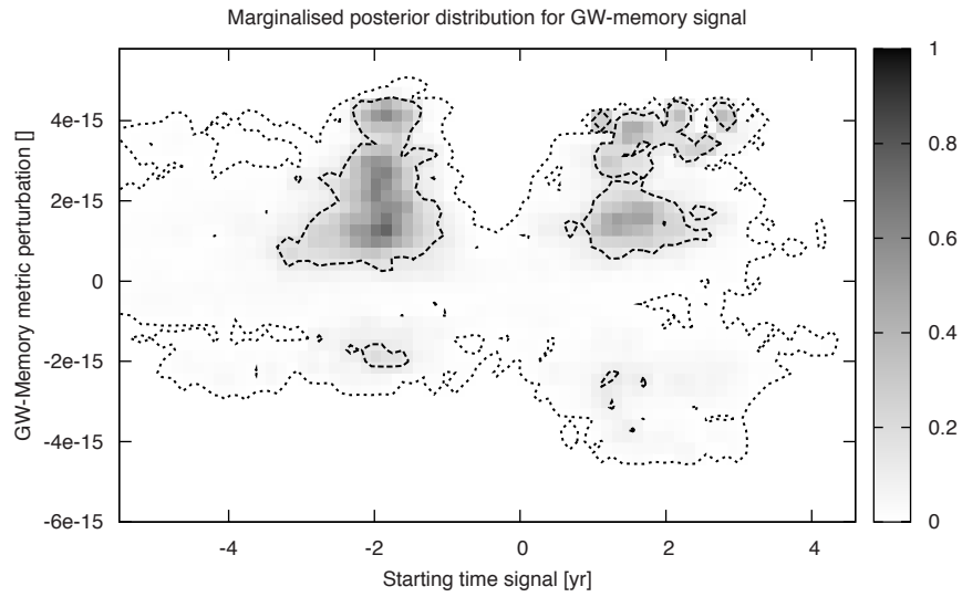
Figure 3.6: The marginalised posterior distribution for the gravitational-wave memory signal amplitude and arrival time of the jump. Here a gravitational-wave signal with an amplitude of 10^{-15} was added to the white residuals. This analysis has been done without marginalising over the EFAC values. The contour drawn is the 3-\sigma contour.
