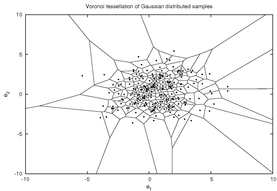
Figure 5.2: An example of a Voronoi tessellation. Here we have taken 200 samples from a 2-dimensional Gaussian distribution as the centres of the Voronoi diagram.
