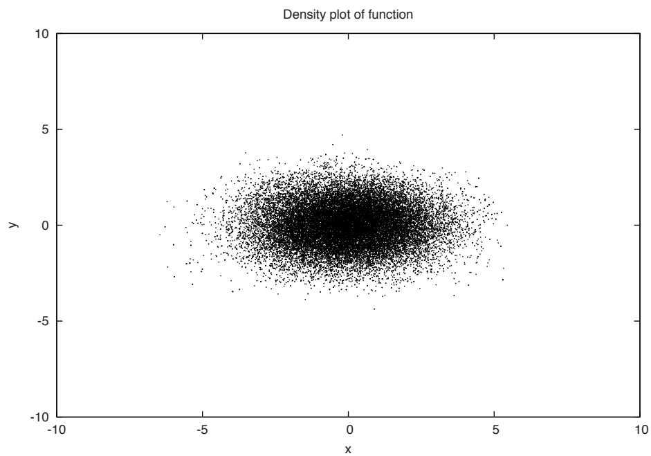
Figure 5.1: A scatter plot of 40000 samples, drawn using a Metropolis algorithm from the function f(x, y) = \exp(-ax^2 - by^2) , with a = 1/5 and b = 2/5 .
