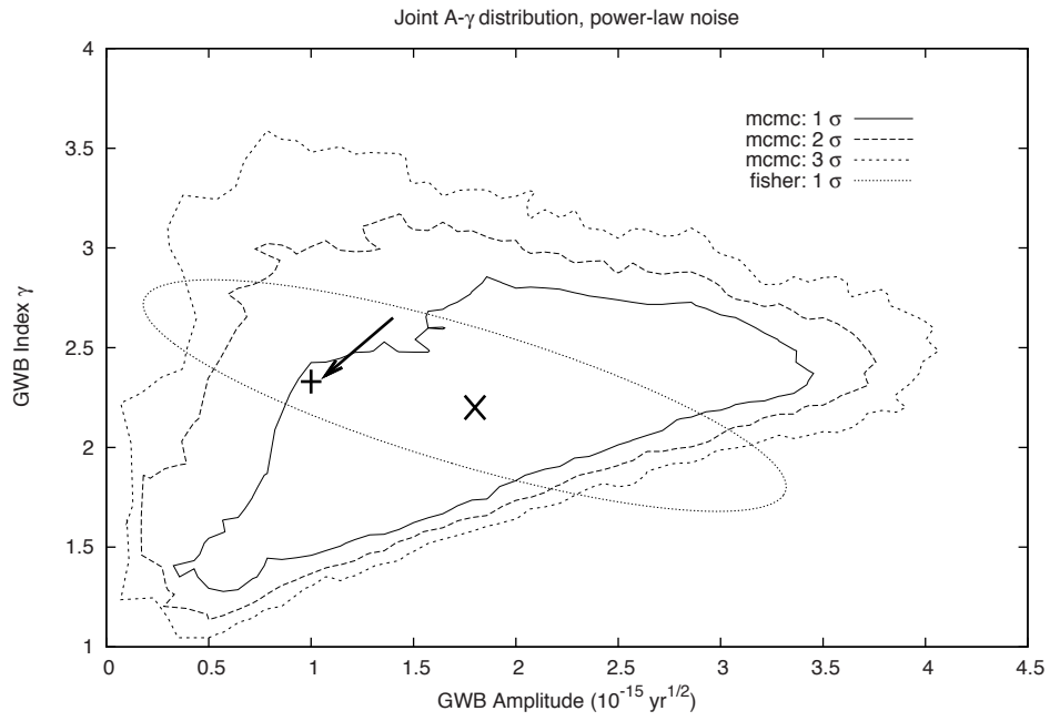
Figure 2.4: Same as in Fig. 2.2, but the mock data is generated and analysed using power law timing noise. Overall timing noise amplitude and spectral index \gamma_i are taken to be 100ns and 1.5 for each pulsar. For all \gamma_i , a prior distribution according to Equation 2.27.
