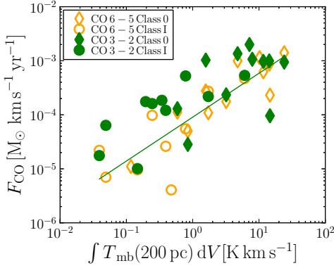
Figure 5.9 – Correlation between F_{\text{CO}} measured from the CO 6–5 and CO 3–2 data and the integrated intensity of the ground-state \text{H}_2\text{O} 1_{10}\text{--}1_{01} transition at 557 GHz. The integrated intensities are scaled to a common distance of 200 pc (Kristensen et al. 2012). The correlation is strong, 3.8\sigma .
