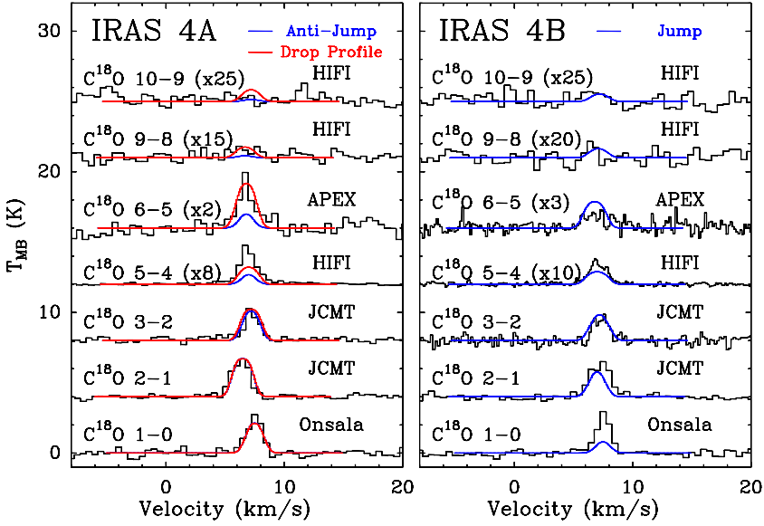
Figure 4.17 – Left : Line profiles obtained with the best-fit anti-jump (blue) and drop abundance (red) envelope models overlotted on the observed \text{C}^{18}\text{O} lines in IRAS 4A. Right : Similar best-fit jump abundance profile for IRAS 4B. See Table 4.8 for best-fit parameters.
