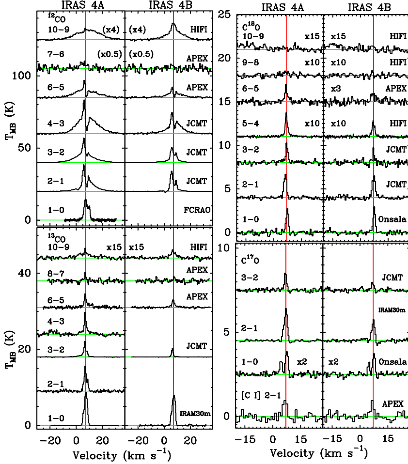
Figure 4.2 — Single spectra obtained from the central positions of IRAS 4A and 4B presented on a T_{\text{MB}} scale. From bottom to top, Left : ^{12}\text{CO} 1–0, ^{13}\text{CO} 2–1, ^{13}\text{CO} 3–2, ^{13}\text{CO} 4–3, ^{13}\text{CO} 6–5, ^{13}\text{CO} 8–7, ^{13}\text{CO} 10–9; ^{12}\text{CO} 1–0, ^{12}\text{CO} 2–1, ^{12}\text{CO} 3–2, ^{12}\text{CO} 4–3, ^{12}\text{CO} 6–5, ^{12}\text{CO} 7–6, ^{12}\text{CO} 10–9; Right : [\text{C I}] 2–1, \text{C}^{17}\text{O} 1–0, \text{C}^{17}\text{O} 2–1, \text{C}^{17}\text{O} 3–2; \text{C}^{18}\text{O} 1–0, \text{C}^{18}\text{O} 2–1, \text{C}^{18}\text{O} 3–2, \text{C}^{18}\text{O} 5–4, \text{C}^{18}\text{O} 6–5, \text{C}^{18}\text{O} 9–8, \text{C}^{18}\text{O} 10–9. The spectra have been shifted vertically for viewing purposes and refer to the observing beams presented in Tables 4.2 and 4.3. The red vertical line corresponds to the source velocity, V_{\text{LSR}} as measured from the \text{C}^{18}\text{O} and \text{C}^{17}\text{O} lines.
