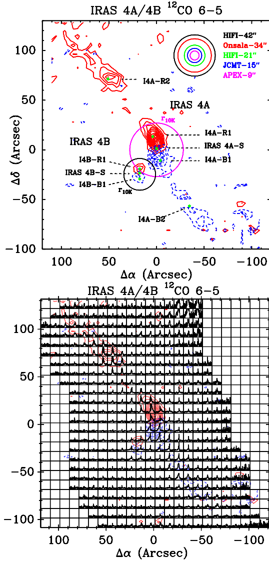
Figure 4.3 – ( Right: ) The ^{12}\text{CO} 6-5 spectral map of IRAS 4A and 4B over the 240'' \times 240'' mapping area. Individual spectra are shown on the T_{\text{MB}} scale from -2 K to 12 K and velocity scale from -20 \text{km s}^{-1} to 30 \text{km s}^{-1} . The outflows of IRAS 4A and 4B are overplotted over the entire spectral map. The map is centered on IRAS 4A. The contour levels start from 3\sigma ( 15 K \text{km s}^{-1} ) with an increasing step size of 2\sigma ( 10 K \text{km s}^{-1} ). ( Left: ) Envelopes of IRAS 4A and 4B at the 10 K radius are shown together with the beam-sizes compared. See Fig. 1 caption and Sect. 3.2.1 for the details and the positions at which deep spectra are obtained.
