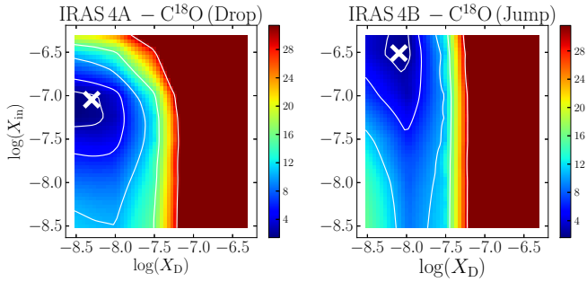
Figure 4.15 – Reduced \chi^2 plots for the drop and jump abundance profile for the \text{C}^{18}\text{O} lines in IRAS 4A and 4B, respectively. The freeze-out abundance X_{\text{D}} and inner abundance X_{\text{in}} were varied. All lines were taken into account except J=1-0 and 5-4 owing to the comparatively larger beam sizes. The contours are plotted at 1\sigma , 2\sigma , 3\sigma , and 4\sigma confidence levels and white crosses show the best-fit values.
