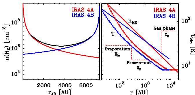
Figure 4.13 – Power-law density profiles discussed for two scenarios in Section 4.3. In the left panel, the IRAS 4A position is taken as the reference and r_{AB} indicates the 4A-4B distance. In the right-hand panel, the individual envelope profiles are shown. This panel includes a typical drop-abundance profile, with an outer abundance X_0 , a freeze-out abundance X_D , and an inner abundance X_{in} . In an anti-jump profile, the evaporation jump in the inner envelope is lacking.
