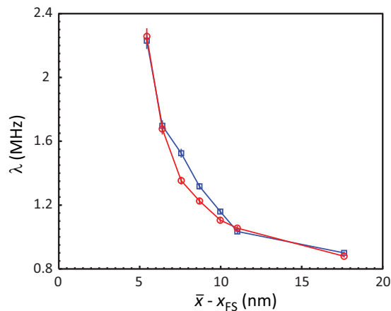
FIG. 3. (Color online) The value of the mean depolarization rate \bar{\lambda}(\bar{x}) obtained from fits to the data using a mean field for each muon implantation energy profile, corresponding to the mean flux density values in Fig. 2. Circles: T = 10 K (Nb in the normal state); squares: T = 4.3 K (Nb in the superconducting state).
