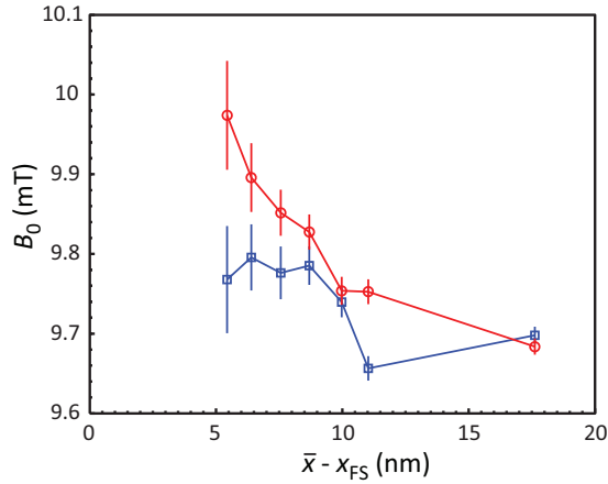
FIG. 2. (Color online) Obtained fit values for the mean flux density B_0 as a function of mean stopping distance inside the superconducting layer, \bar{x}(E) - x_{FS} , with x_{FS} being the position of the left-hand (topmost) Py/Nb interface (see Fig. 1). Circles: T = 10 K (Nb in the normal state); squares: T = 4.3 K (Nb in the superconducting state).
