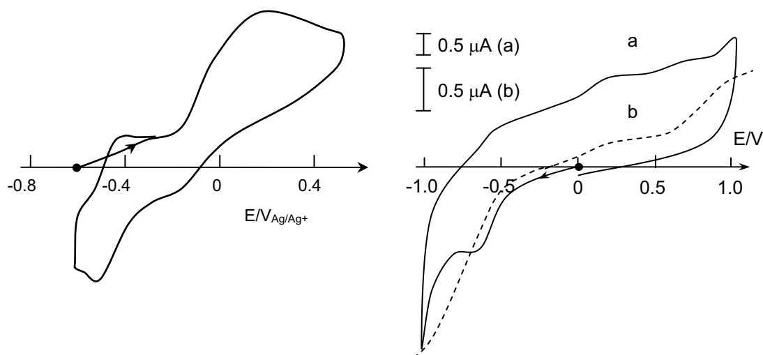
Figure 7.5. Left: CV curve recorded in a 1 mM solution of 2 in \text{CH}_3\text{CN} + 0.1 M TBAP on a Pt disc ( \varnothing = 5 mm), v = 0.1 \text{V}\cdot\text{s}^{-1} . Right: voltammetric curve in \text{CH}_3\text{CN} + 0.1 M TBAP of the peroxo-dicopper complex 3 ( in situ , 2.5 \times 10^{-4} M, \text{CH}_3\text{CN} , -40 °C). (a) CV curve 0.1 \text{V}\cdot\text{s}^{-1} (b) (dotted line) RDE 6000 rpm. E vs. \text{Ag}/10 mM \text{AgNO}_3 + 0.1 M TBAP in \text{CH}_3\text{CN} .
