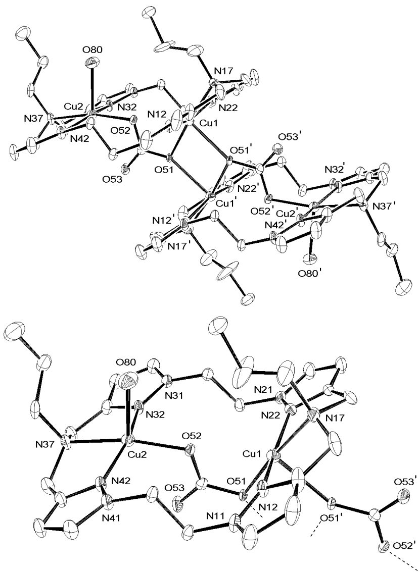
Figure 8.3. ORTEP projection of the tetranuclear cation [\text{Cu}_2([\text{22}]pr_4pz)(\text{CO}_3)(\text{H}_2\text{O})]_2^{4+} ( (\mathbf{I})_2^{4+} ) (top) and ORTEP projection of half of the tetranuclear cation ( \mathbf{I}^{2+} ) (bottom). Hydrogen atoms and solvent molecules are omitted for clarity. Symmetry operation ' : 2-x, y, 0.5-z .
