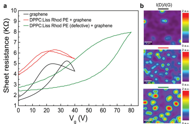
Fig. 5 (a) The back gate voltage ( V_g ) dependent sheet resistance ( R ) of graphene on \text{SiO}_2/\text{Si} substrate (black line), lipid–graphene assembly (red line), and of graphene with defective lipid monolayer (green line). (b) Raman imaging of the intensity ratio of I(D)/I(G) for graphene on \text{SiO}_2/\text{Si} substrate (top), lipid–graphene assembly (middle), and graphene with defective lipid monolayer (bottom).
