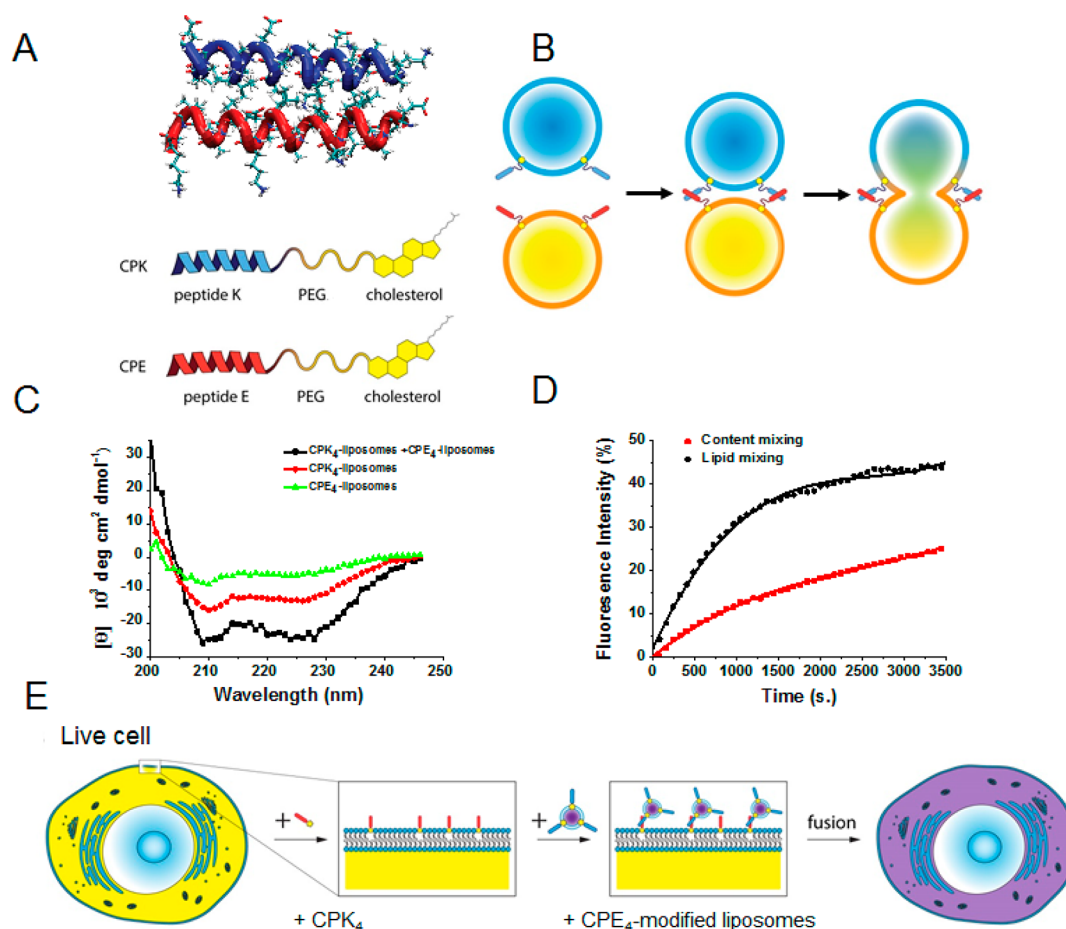
Figure 1. Schematic representation of (A) coiled-coil structure between peptides E and K (adapted from PDB 1U01), (B) targeted liposome fusion mediated by coiled-coil formation between CPE 4 modified liposomes and CPK 4 modified liposomes, (C) CD spectra of CPE 4 modified liposomes, and CPK 4 modified liposomes and an equimolar mixture thereof. The total lipid concentrations were 0.5 mM with 1 mol % of lipidated peptide in PBS. (D) Lipid mixing and content mixing between CPE 4 -liposomes and CPK 4 -liposomes. Fluorescence traces showing lipid mixing between E and K decorated liposomes, as measured through an increase in NBD fluorescence. Total lipid concentrations were 0.1 mM with 1 mol % of lipidated peptide, in PBS; fluorescence graphs indicating content mixing between sulphorhodamine loaded (20 mM), CPE 4 decorated liposomes and nonfluorescent, CPK 4 decorated liposomes. Total lipid concentrations were 0.25 mM with 1 mol % lipidated peptide in PBS. (E) Scheme of fusion between cell and liposomes.
