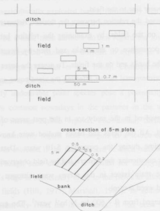
Fig. 1. Diagram (not to scale) showing the location of the vegetation sampling plots on the field and the ditch banks (hatched). Both the 50-m and the 5-m ditch bank plots are indicated; in a cross-section of the latter the distinguished strips are indicated.
