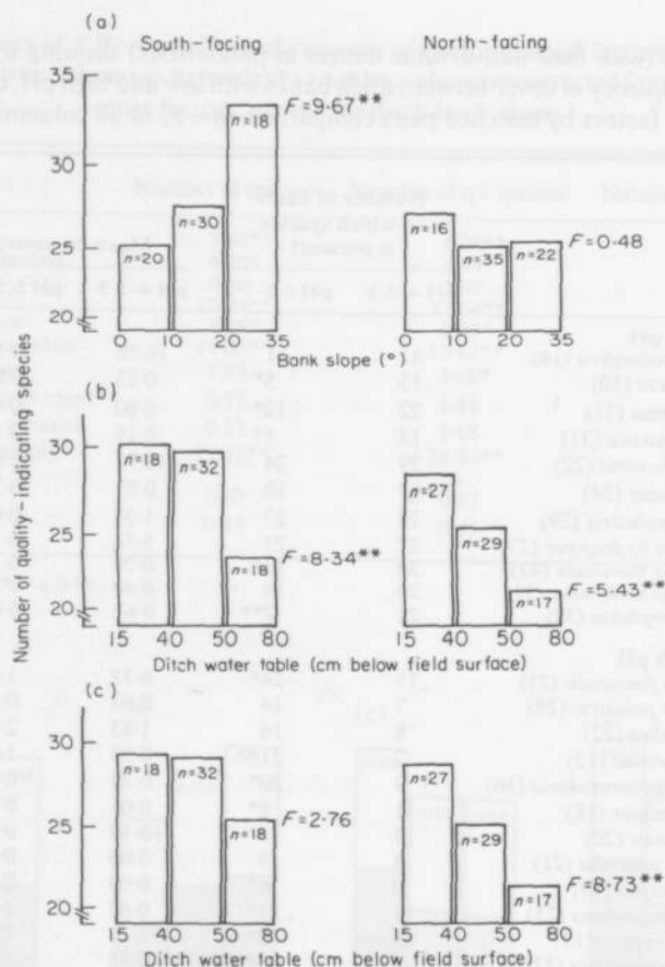
FIG. 3. Effects of ditch bank slope and ditch water table on the number of quality-indicating species on south- and north-facing slopes: (a) effects of ditch bank slope; (b) effects of ditch water table; (c) overall effects of ditch water table. All corrected for other factors, except (c) was not corrected for ditch bank slope ( ^{**} P < 0.01 ).
