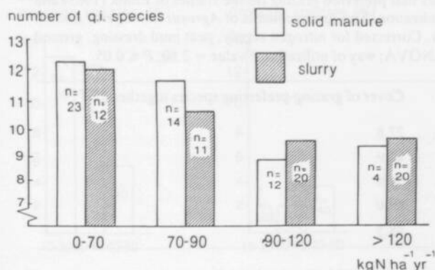
Fig. 6. Average number of quality-indicating species on fields treated with different doses of manure or slurry. Corrected for effects of fertilizer treatment, excreta deposited during grazing, peat mud dressing and soil type by means of ANOVA. The doses of both types of animal manure have been converted into amounts of effective nitrogen supply.
