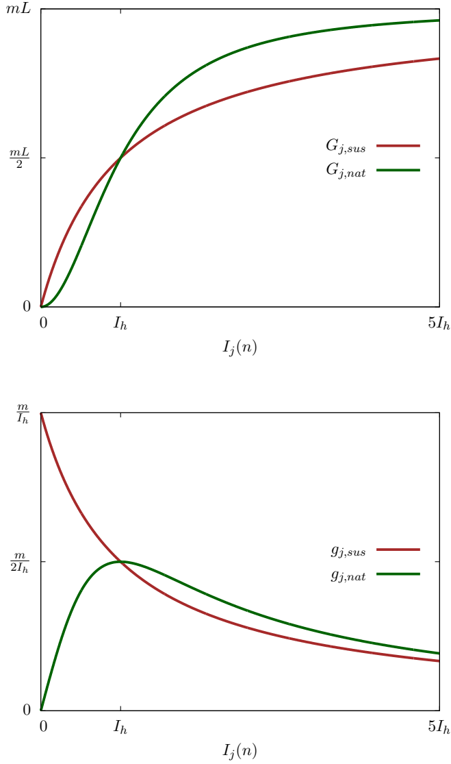
Figure 4.2: Grazing as a function of available forage I_j(n) . Here I_h designates the amount of forage where the total grazing is half the maximum value and m = m_{\text{sus}} or m_{\text{nat}} respectively. Note that the graphs do not depend on j . Top panel: in both cases the total grazing G converges to mL as forage becomes more and more abundant and diminishes if vegetation becomes scarce. Bottom panel: in both cases the grazing pressure g is (approximately) inversely proportional to available forage in case of abundant forage. The function g_{j,\text{sus}} monotonically increases to m/I_h as all vegetation disappears; in contrast g_{j,\text{nat}} initially increases to a maximum at I_j(n) = I_h but then converges to zero for ever smaller forage amount.
