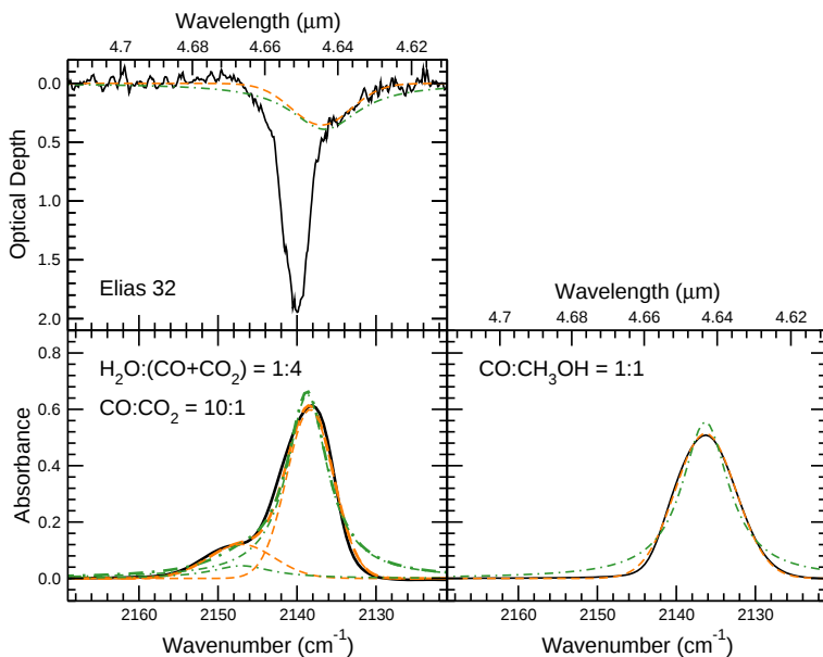
Figure 4.2 – A comparison between fits of the red CO-ice profile by Gaussian line shapes (dashed curves) and by Lorentzian line shapes (dash-dotted). (Top) The Gaussian fit yields the best-fit result for Elias 32 and is used in this study; the Lorentzian result is taken from Pontoppidan et al. (2003b).
