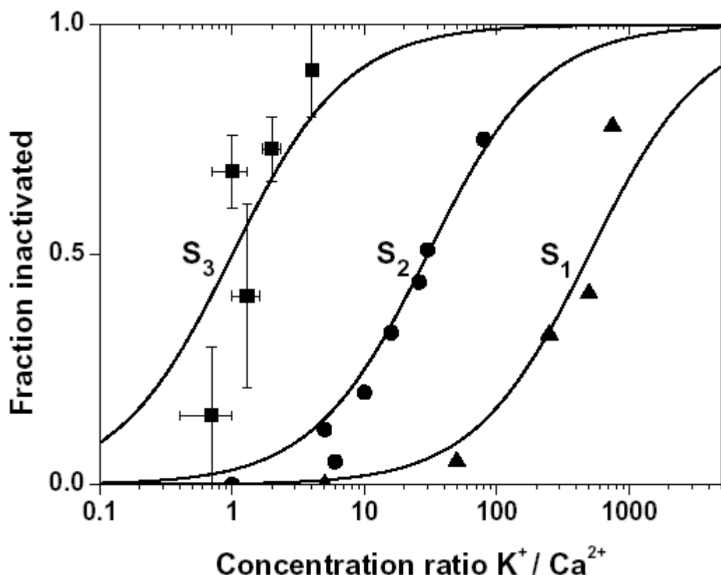
Figure 4. Extent of inhibition versus the ratio of added K^+ and Ca^{2+} concentrations in experiments as shown in Fig. 3. The lines are fits assuming a binding competition at a single site with an S-state dependent K_d ratio, yielding values of 500, 30, and 1 for S_1 , S_2 , and S_3 , respectively. See text for the error bars in the case of S_3 .
