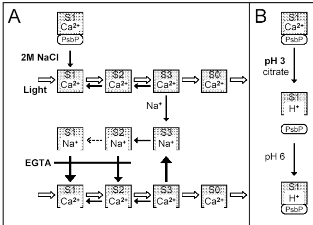
Figure 2. \text{Ca}^{2+} depletion by the salt-wash (A) and low pH (B) methods. The diagram illustrates this process starting from PSII membranes in \text{Ca}^{2+} free medium. Both treatments release PsbP and PsbQ from PSII, displace \text{Ca}^{2+} from its binding site, and modify the site so that in the case of salt-washing, it exchanges metals rapidly. During salt-treatment (A), this process depends on the \text{Na}^{+}/\text{Ca}^{2+} concentration ratio as well as on the S-state, \text{S}_3 having most rapid exchange rate. Exchange is much slower than the \text{S}_3 lifetime, so that prolonged illumination (open arrows) is required to trap all PSII centers in the stable \text{S}_2(\text{Na}^{+}) state. If no chelator (for example, EGTA) is added, subsequent centrifugation and resuspension in low-salt medium decreases the \text{Na}^{+} concentration much more than the residual \text{Ca}^{2+} concentration and may cause rebinding of \text{Ca}^{2+} (bottom line). The resulting preparation is then active and shows normal behavior in single-turnover experiments, but its maximum \text{O}_2 evolution rate may be much decreased by the accumulation of \text{S3}(\text{Na}^{+}) during illumination, because the \text{Ca}^{2+} site remains in fast exchange (seconds, heavy arrows). After low pH treatment (B), \text{Ca}^{2+} rebinding is avoided by the presence of citrate and by rebinding of PsbP.
