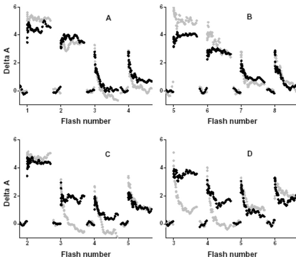
Figure 2. S-state dependence of \text{Cd}^{2+} accessibility and substitution for \text{Ca}^{2+} in PSII membranes depleted of PsbP and PsbQ, but not \text{Ca}^{2+} , by pH 7.5 / sulfate treatment. Absorbance changes were measured at 295 nm as in Fig. 1. but in the presence of 15 mM \text{CaCl}_2 , and with 100 \mu\text{M} DCBQ as electron acceptor. The first 4 flashes after addition of 5 mM \text{CdCl}_2 are shown, in A and B (low S-states) 30 s after addition; in C and D ( S_2 and S_3 ) 5 s after addition.
