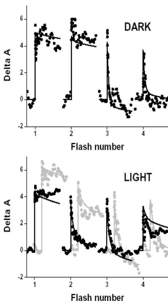
Figure 2. The effect of 70 mM CaCl 2 added immediately (2-3 seconds) before a flash series, on absorbance changes at 295 nm. Conditions are given in Fig. 1. Upper frame: KCl-treated in the dark. Lower frame: samples incubated with KCl in darkness and then in room light. Grey traces: Identical conditions, but with a 10 s delay between CaCl 2 addition and initiation of the flash series. The lines represent a global fit to the Kok model (see text).
