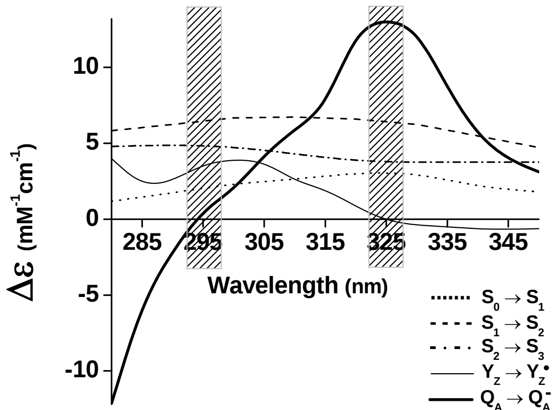
Figure. 1. Absorbance difference spectra of S-state transitions, Y_Z oxidation, and Q_A reduction. Grey bars show the half width of the spectral profile of the measuring light used here, which was centered either at 295 or at 325 nm to minimize Q_A or Y_Z contributions, respectively. Based on data from van Leeuwen et al. (1993) and Dekker et al. (1984b).
