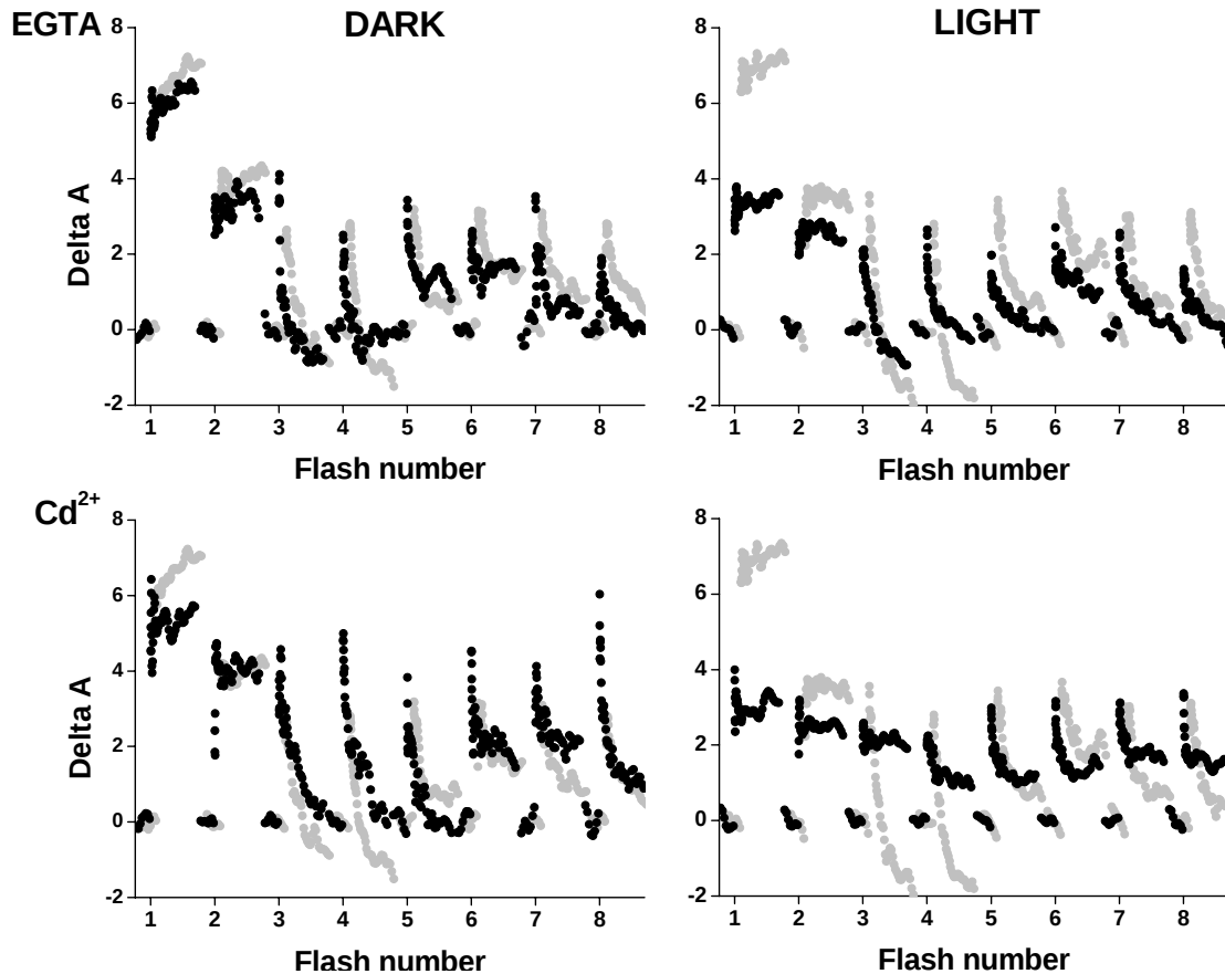
Figure 1. The effect of a saturating concentration of 20 mM EGTA (upper frames, black traces) and 15 mM \text{Cd}^{2+} (lower frames, black traces) added 5 seconds before measurement of flash-induced absorbance changes at 295 nm in PSII membranes that had been \text{Ca}^{2+} -depleted by exposure to 1 M KCl / 1 mM EGTA either for 30 min in the dark (left frames), or for 30 min in dark and 30 min in room light (right frames), and then reactivated by incubation for at least 5 min with 4 mM CaCl before the experiments (gray traces). Flash frequency 4 Hz. Absorbance changes were recorded from 20 ms before to 50 ms after each flash. Concentrations: 200 \mu\text{g} Chl/ml, in 50mM MES, 0.4 M Sucrose, 30 mM TMAC, 30 mM Betaine, 100 \mu\text{M} PPBQ. Delta A units correspond to differential extinction coefficient \text{mM}^{-1}\text{cm}^{-1} assuming 250 Chl/PSII.
