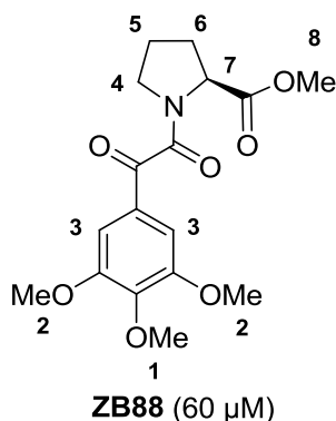
Figure 2.3 : 1D- 1 H NMR spectra of ZB88 in the free form (top trace), and in the presence of diamagnetic FKBP12 (34/35-Lu, middle trace) and paramagnetic FKBP12 (34/35-Tm, bottom trace). The proton assignments correspond to the numbers on the ligand structure, with K_D in brackets (left). Signal intensities were scaled non-linearly for ease of viewing the shapes of the resonances. Asterisks indicate the protein/buffer resonances. [FKBP12]=75 \mu M, [ZB88]=2000 \mu M, resulting in a ligand : protein ratio of 26.7 and a bound ligand fraction of 3.6%. The T_2 filter was 50 ms.
