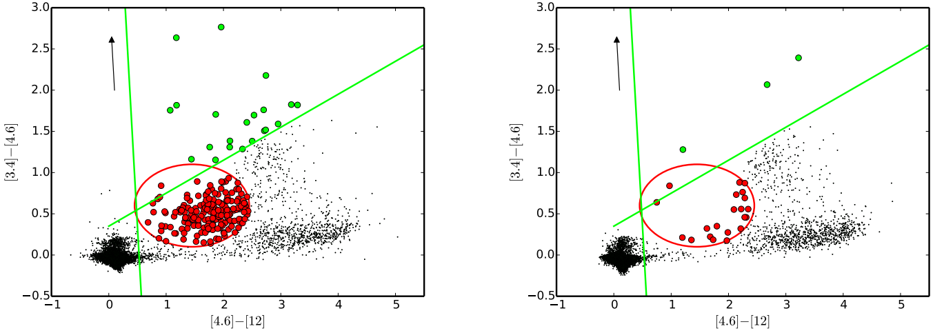
Fig. 11. W1–W2 ([3.4]–[4.6]) vs. W2–W3 ([4.6]–[12]) diagram for the science and the control field. Red points represent candidate Class II objects, green points represent candidate Class I objects, while black points represent the other sources in the field. The red ellipse and the green lines have equations specified in the text.
