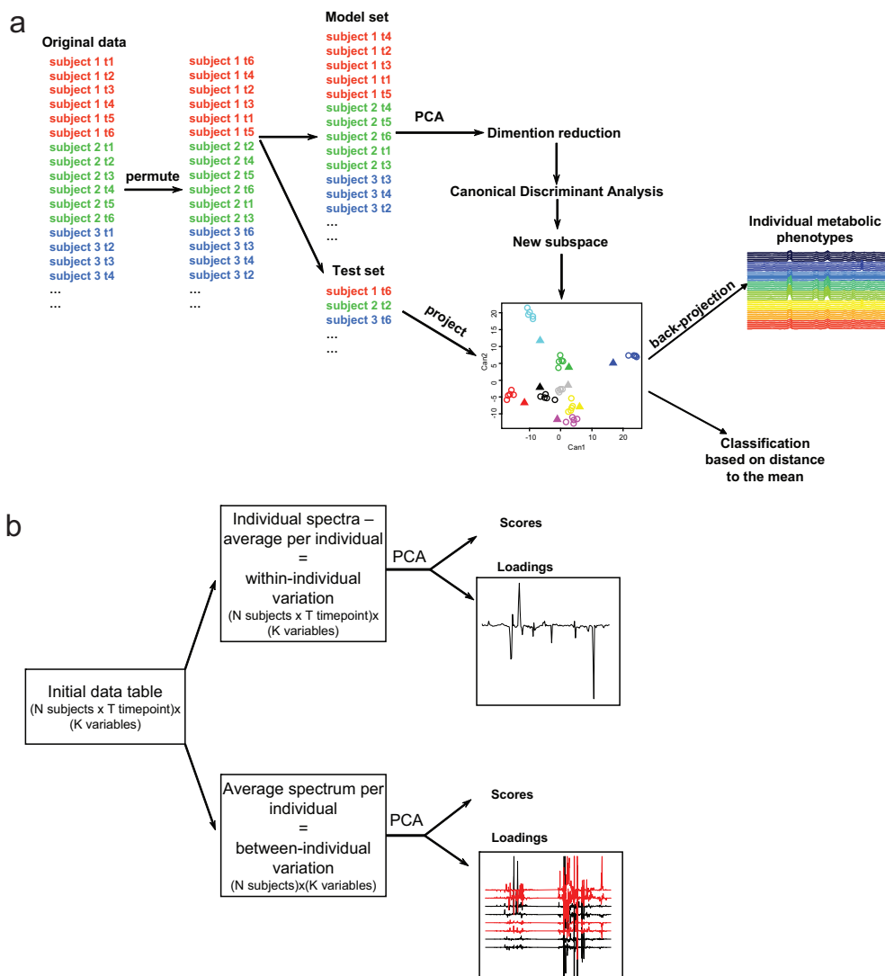
Figure S3. Schematic representation of the two statistical methods used: (a) person recognition, (b) multilevel component analysis.
