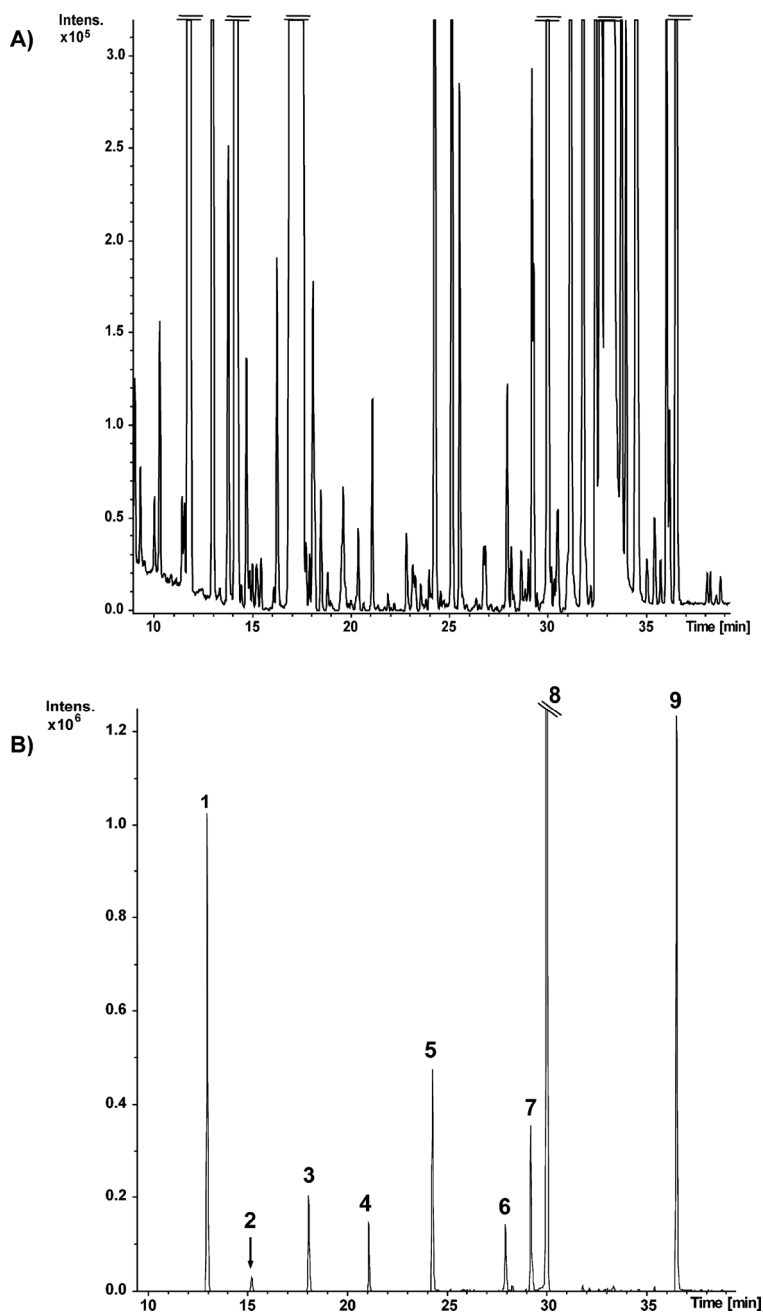
Figure 2. GC/APCI-TOF MS analysis of CSF sample: (A) Base peak chromatogram of the derivatized CSF sample. (B) EICs of several identified metabolites; peaks 1 (Glycine), 2 (Uric acid), 4 (Threonine) assigned with help of standards, peaks 3 (Glycerol), 5 (Pyroglutamic acid), 6 (N-acetyl-aspartate), 7 (Ribitol), 8 (Glutamine), 9 (Glucose) assigned using mass position and isotopic pattern.
